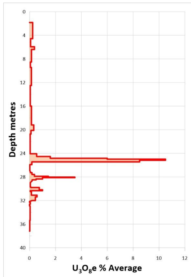
Figure 2: Graph of the high-grade uranium intersection (non-JORC), showing radiometric calculated uranium values (see table 2) completed in 1968 by the Big Horn Mining Company from the Big Horn DH diamond cored drillhole (Erickson, October 1968).
