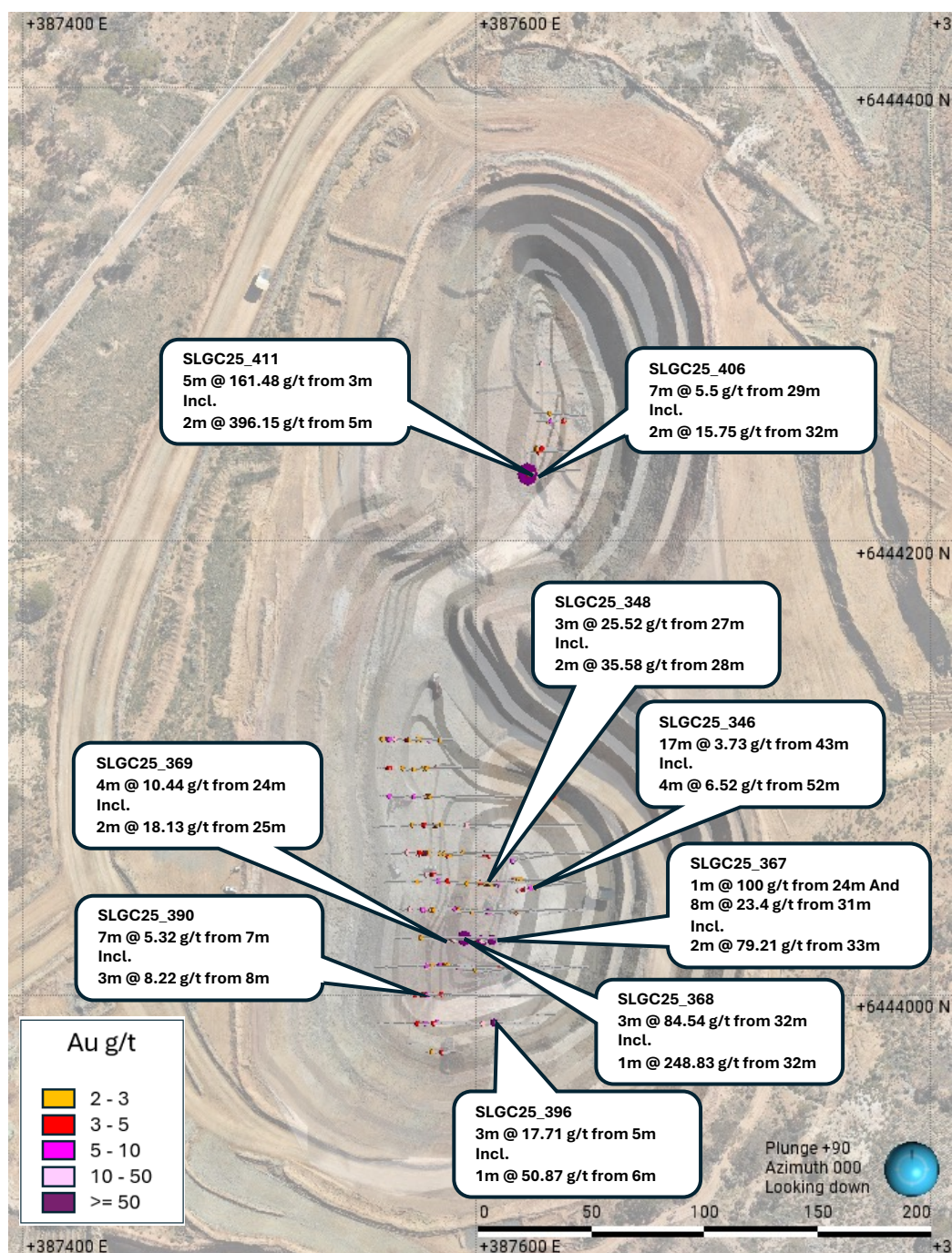
Figure: Plan view of Slippers Open Pit grade control drilling.
