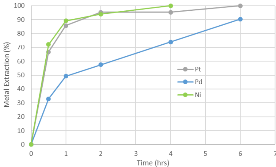
Figure 2 – Leach Kinetic Curves for Sample Number 1
