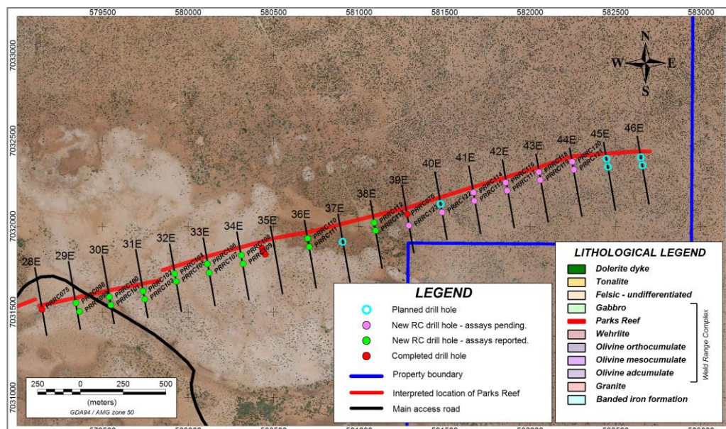
Figure 2 – Resource drilling sections and hole location plan
