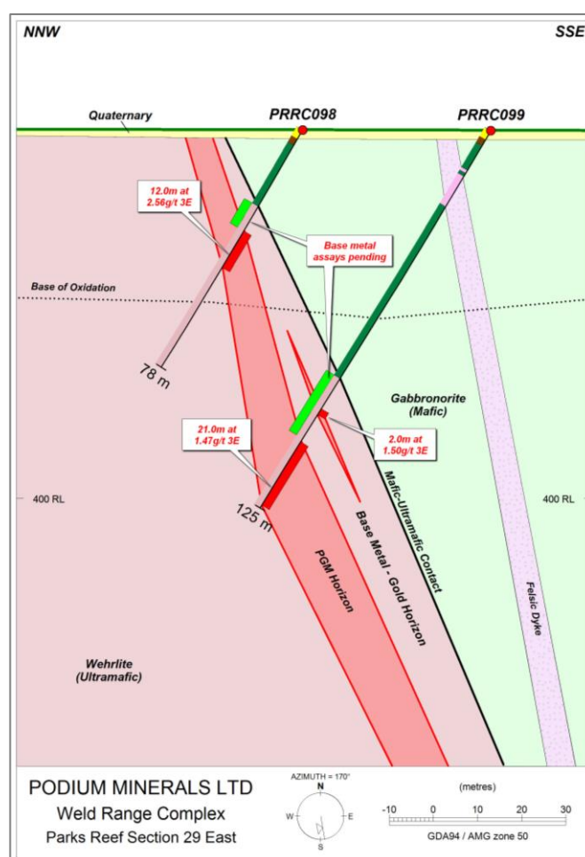
Figure 3 – Drill hole cross section 29 East
