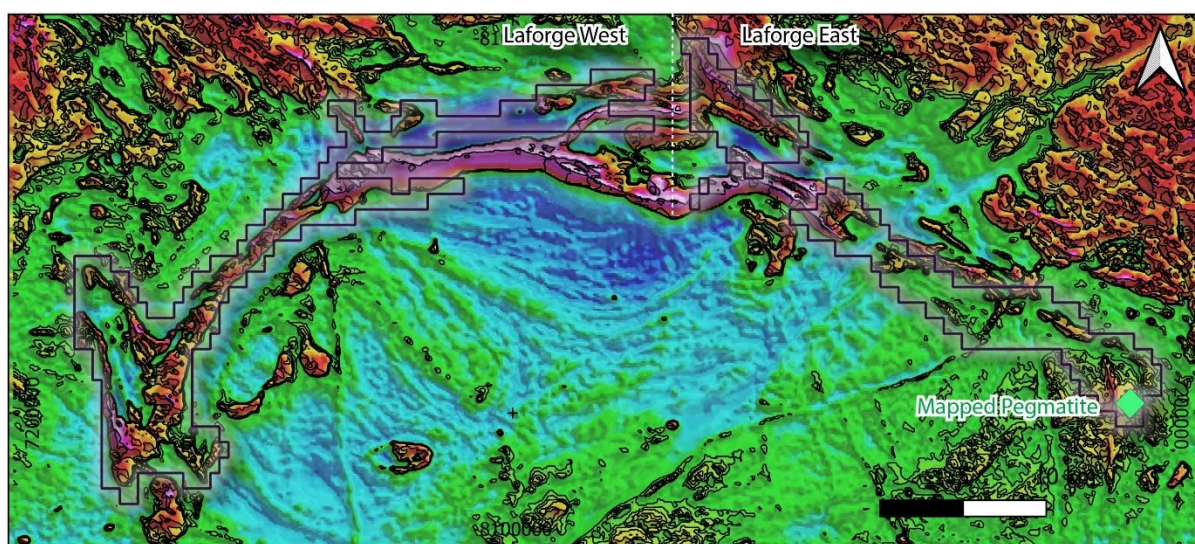
Figure 3: Magnetic image of PR1 (Canada) Ltd Laforge claims highlighting the high-magnetic, primary target corridors. Scale 1:550,000
