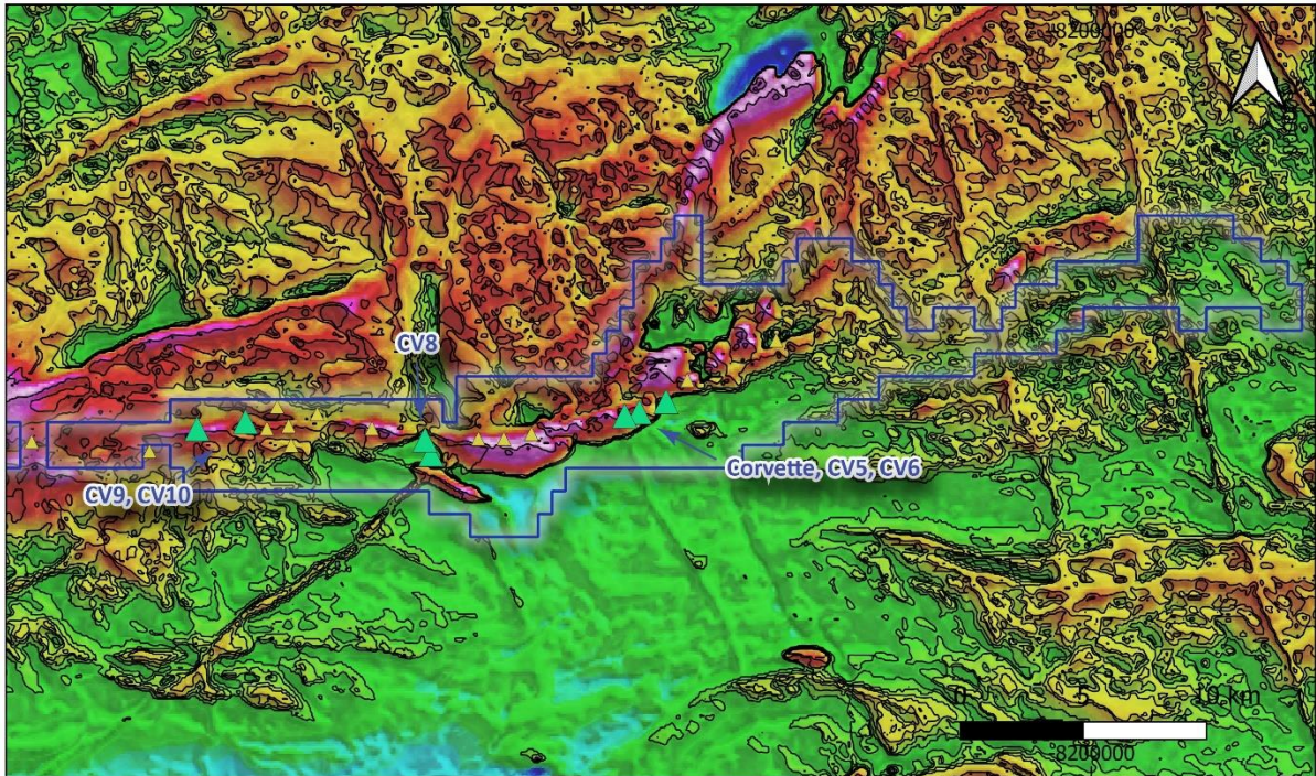
Figure 4: Magnetic image of Patriot Battery Metals Inc. Corvette property highlighting the high-magnetic, primary target corridors. Scale 1:400,000
