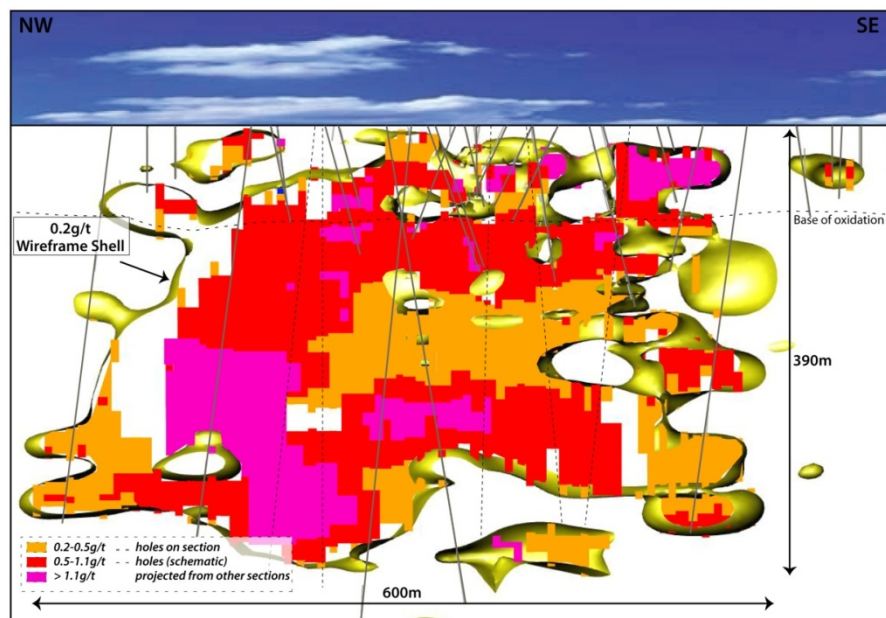
Long Section
