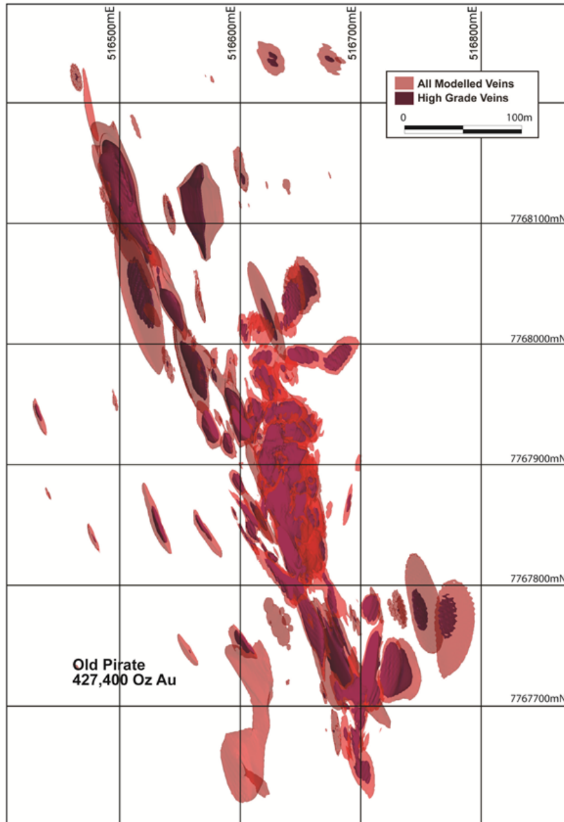
Figure 2. Plan view of the Old Pirate Grade / Vein Shell Model.
