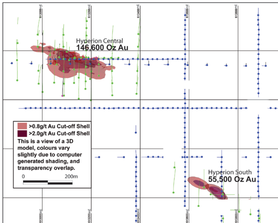
Figure 12. Hyperion Central and South grade shell models (green lines RC drilling, blue lines RAB and Vacuum Drilling).
