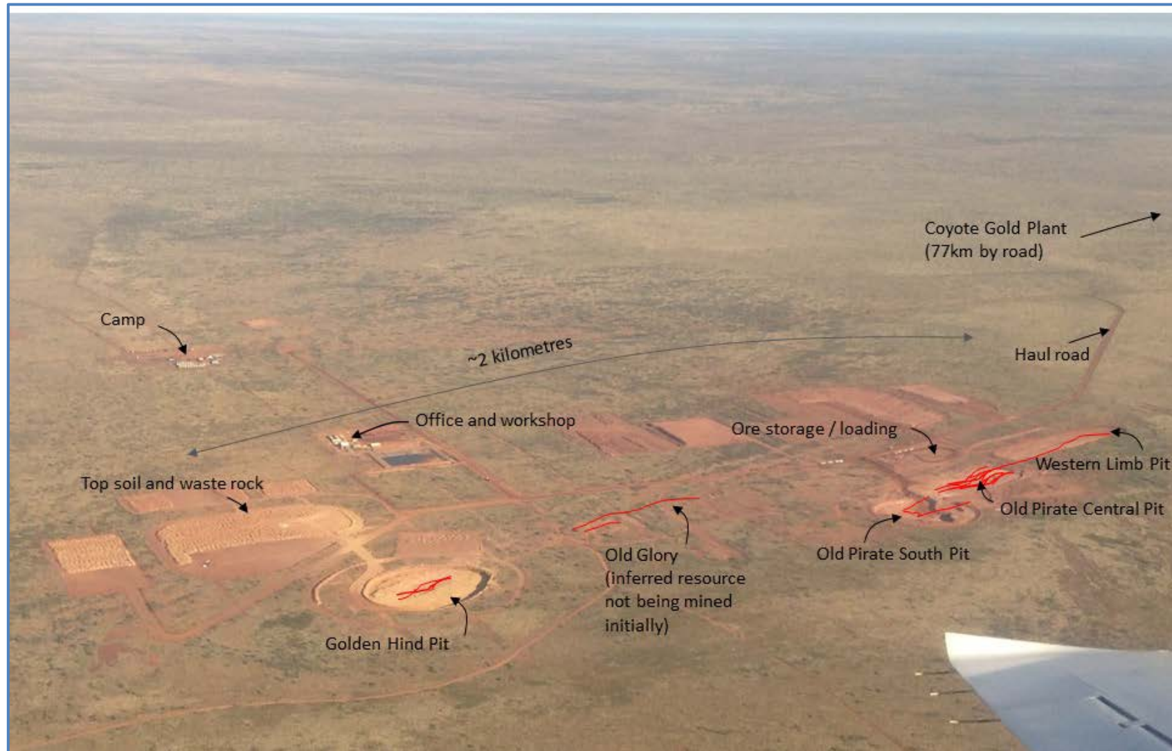
Figure 2. Site layout aerial photograph on 12/05/2015. Red lines indicate approximate location of high-grade gold bearing quartz veins. View west
