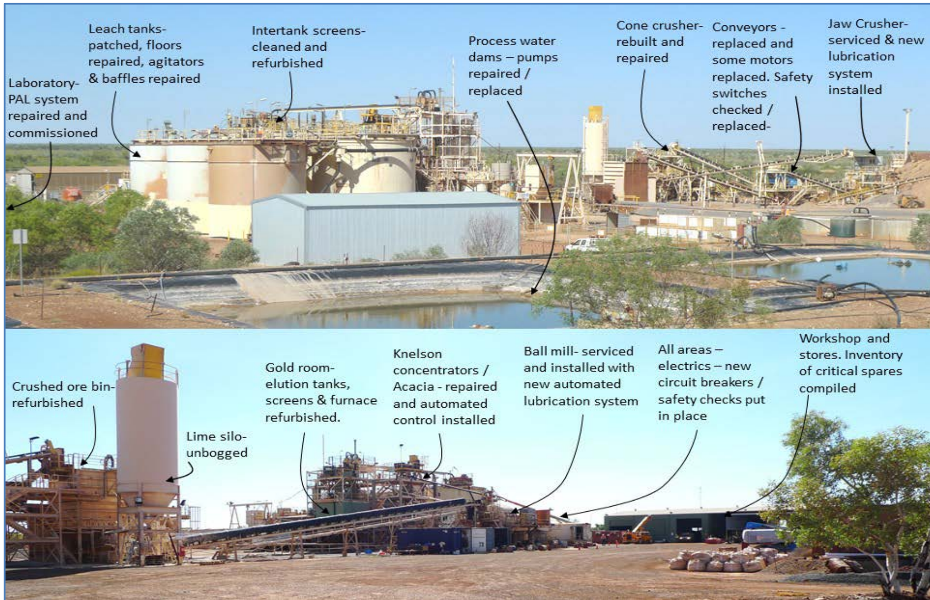
Figure 3. Coyote Gold Plant refurbishment nearing completion. Top image is view to southeast and bottom image is view to northwest
