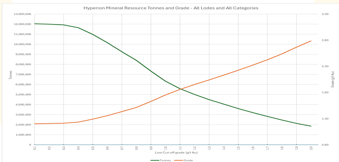
Figure 9 Tonnes and Grade Graph for the Hyperion Mineral Resource
