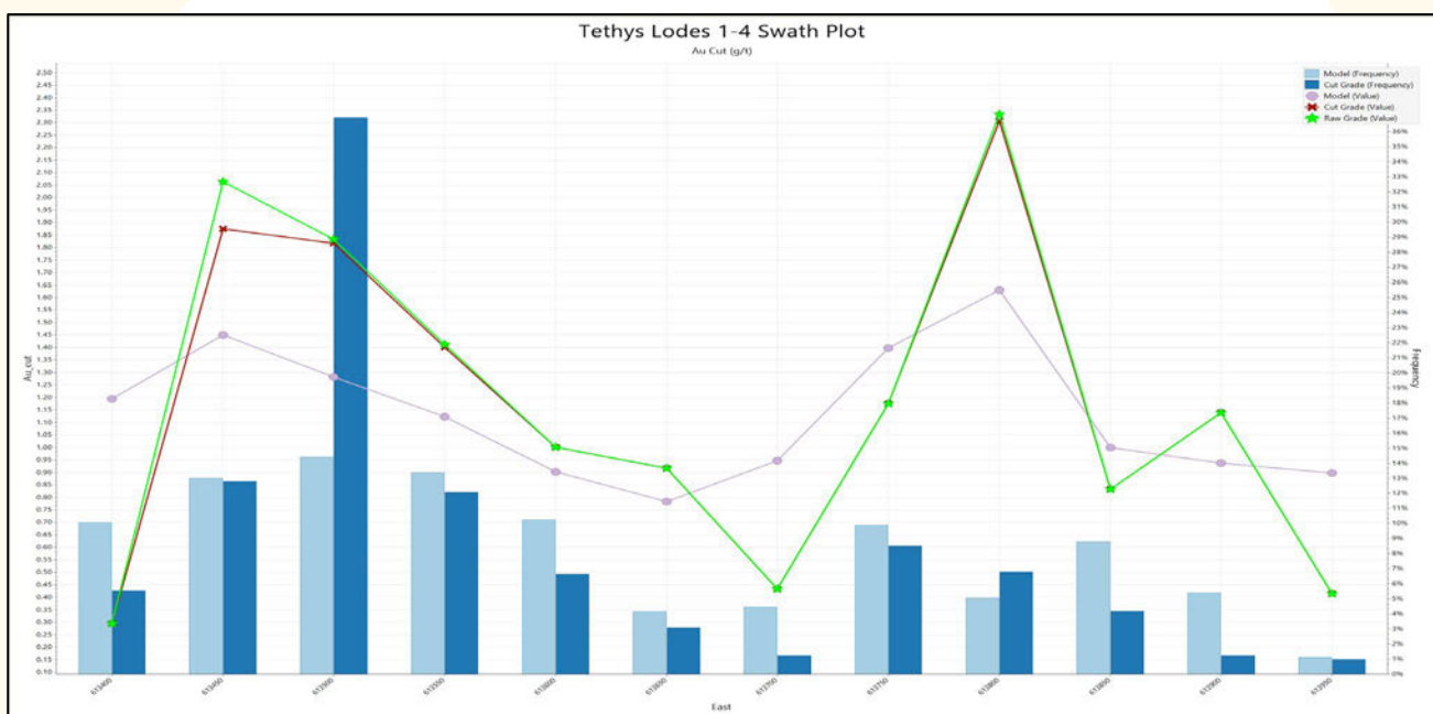
Figure 8 Example Swath Plot of Tethys Lodes 1-4
