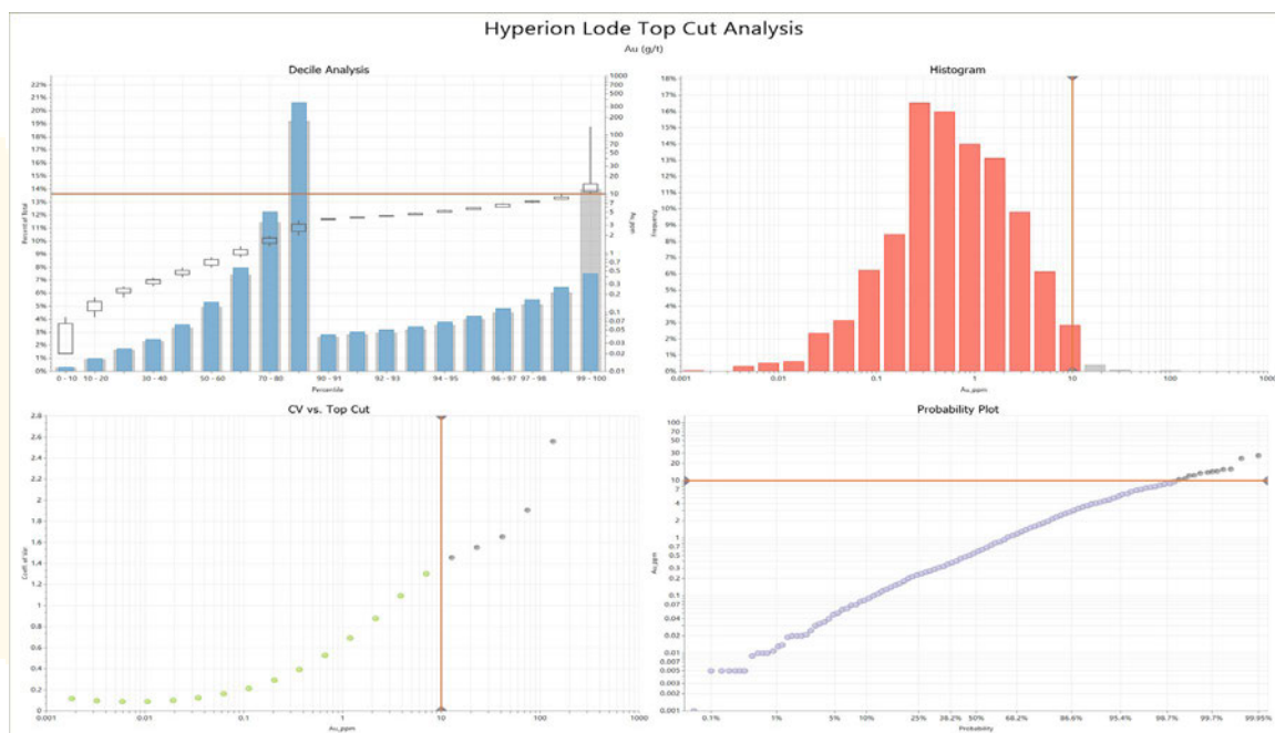
Figure 6 Top-cut analysis for the Hyperion mineralised lodes
