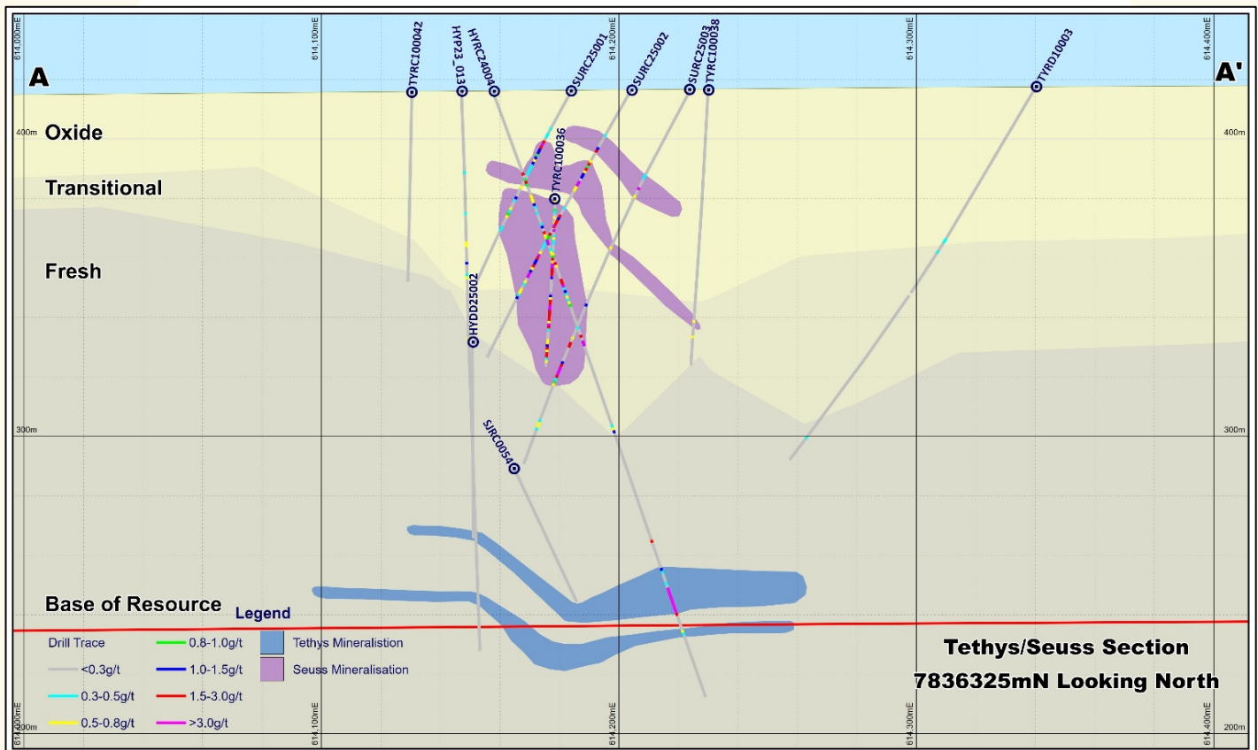
Figure 5 Section through Seuss and Tethys mineralisation looking north
