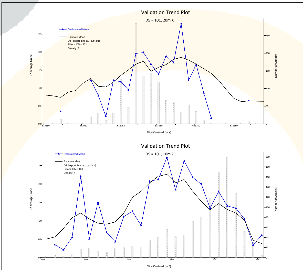
Figure 6 Validation by 20m Strike Panel & 10m Elevation, Domain 101 (Black=Block OK, Blue=Declustered Composite Grade)
