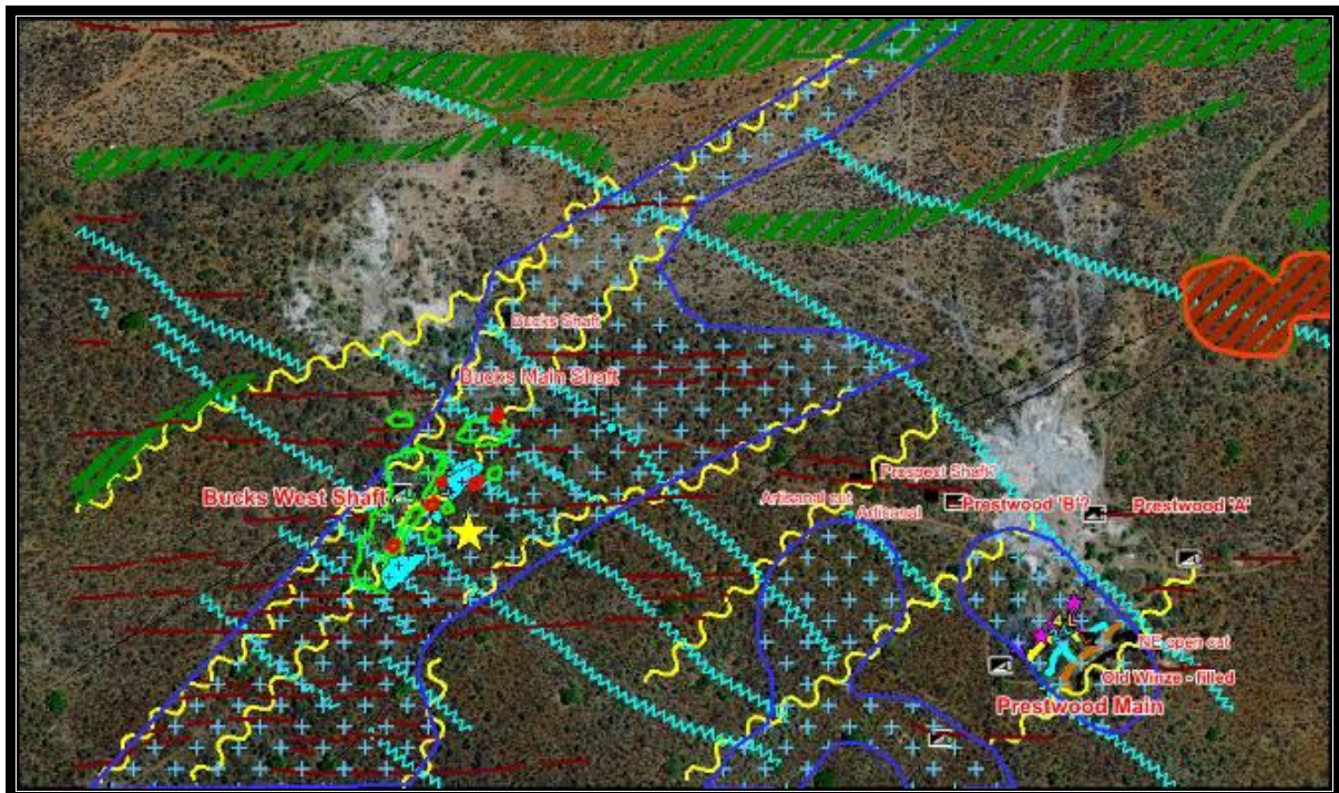
Figure 3: Position of the current artisanal activity (yellow star) superimposed on the geological model. The newly active artisanal zone extends for almost 200m along a shear
