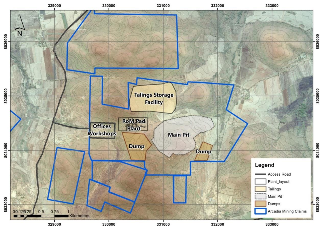
Figure 2 – Arcadia Project Infrastructure and Layout
