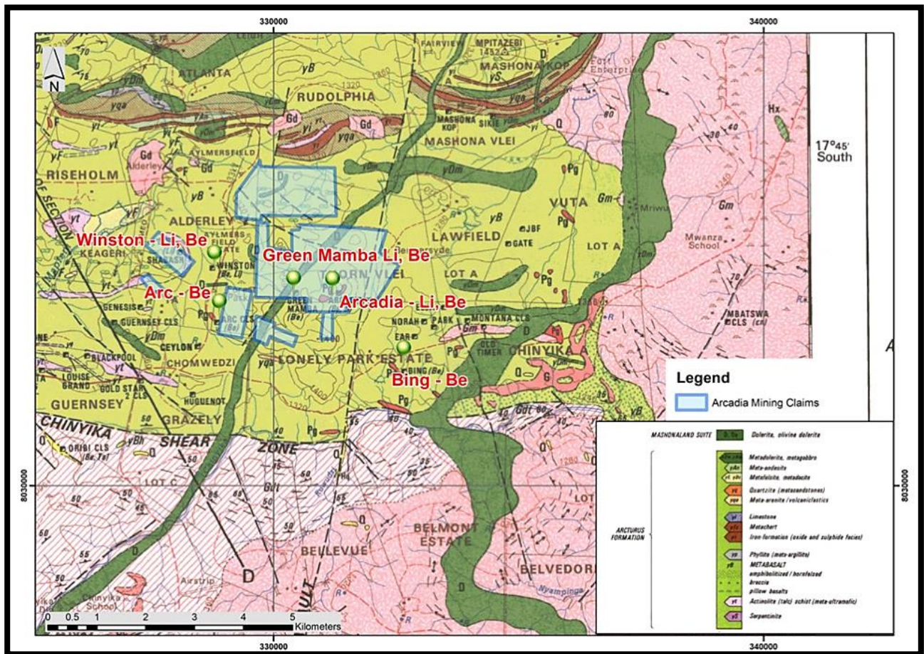
Figure 3 The Arcadia Lithium Project and Prospect Resources Ltd tenure overlain on the regional geology
