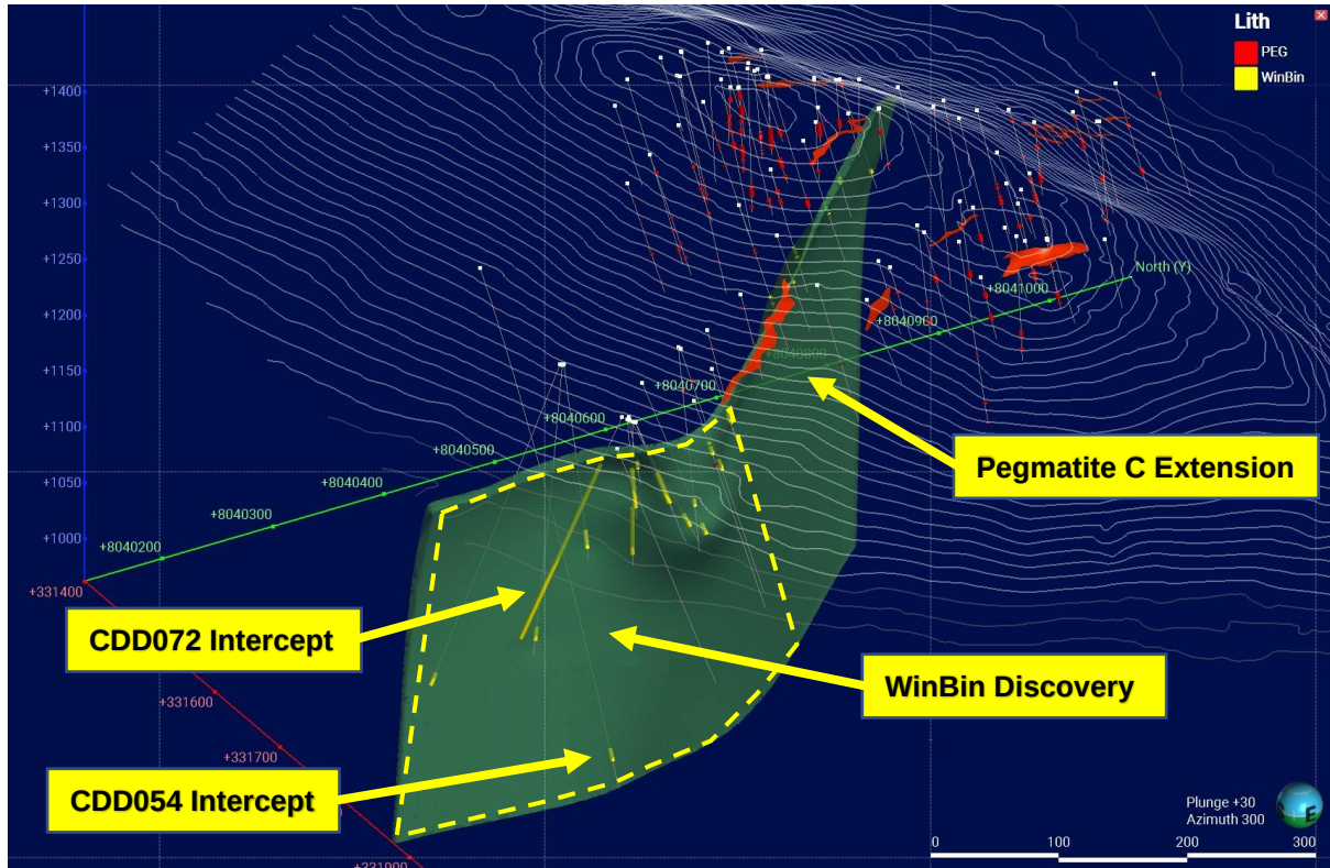
Figure 2: 3D oblique projection of combined WinBin/Pegmatite C extension looking northwest
