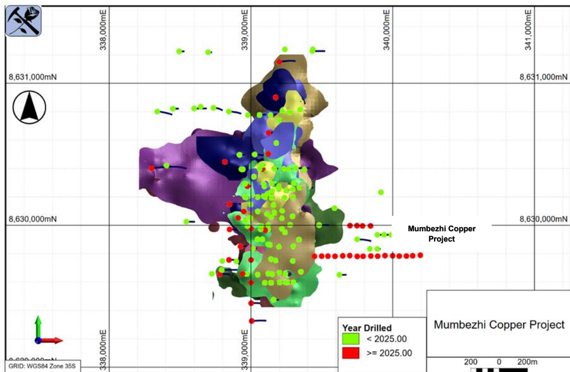
Figure 9: Plan view showing mineralisation wireframes for Nyungu Central prospect
