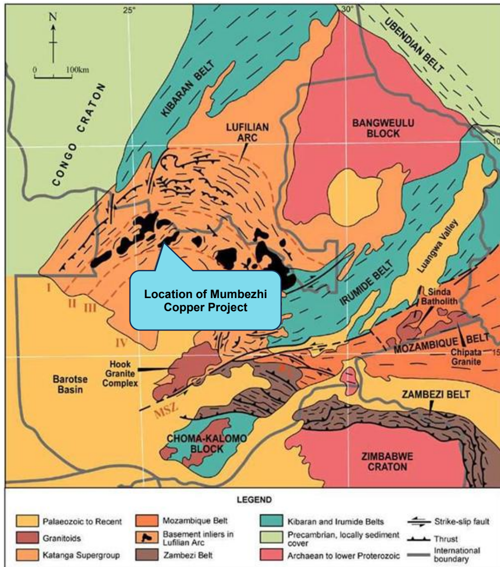
Figure 4: Regional Geological Setting of the Mumbezhi Copper Project in Northwest Zambia (grid lines shown in Latitude and Longitude)
