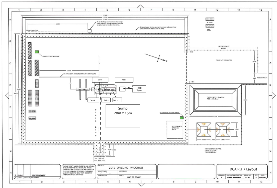
Site layout for DCA Rig 7 including the layout of surface casing and drill pipe (below)
