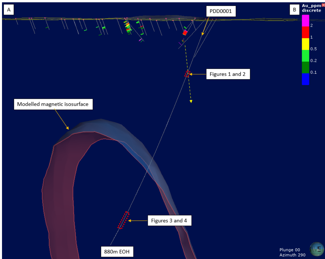
Figure 6: Section A-B. Drill hole trace of EIS diamond drillhole PDD0001 showing the approximate location of the photographs in Figures 1-4.
