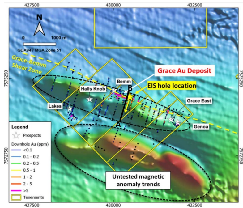
Figure 5: Magnetic intensity map covering the Grace and Bemm Shear zone trend, showing two large untested magnetic anomaly trends, the location of the completed EIS co-funded deep diamond drillhole, historical gold drilling, and the outline of the Company's 100% owned mineral prospecting tenements. Section A-B shown in Figure 6.
