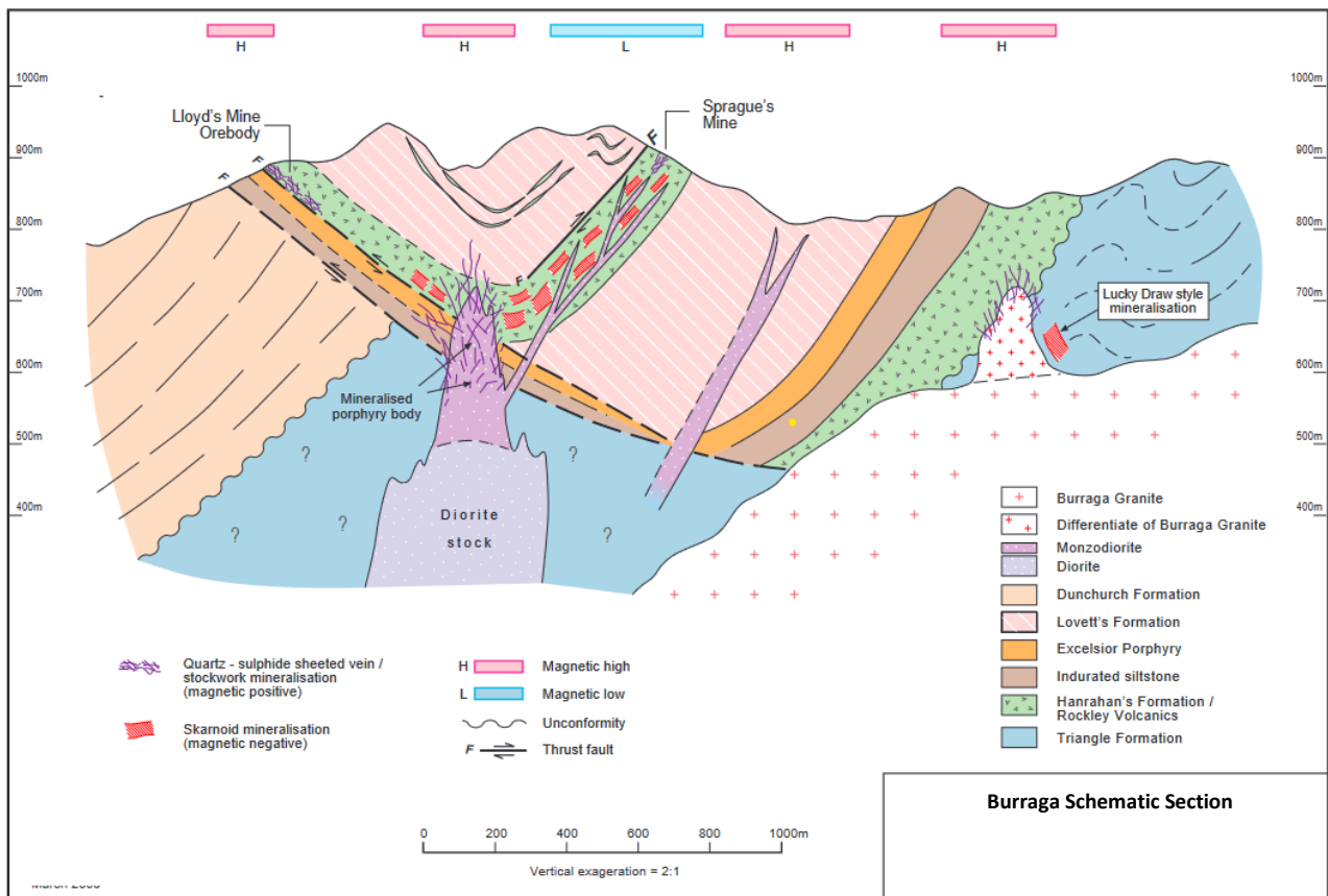
Figure 1: Geological model for the formation of copper-lead-zinc-gold mineralisation at Burrage
