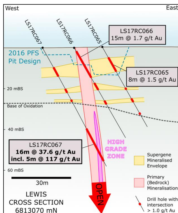
Figure 2: Cross section showing recently announced results at Lewis
