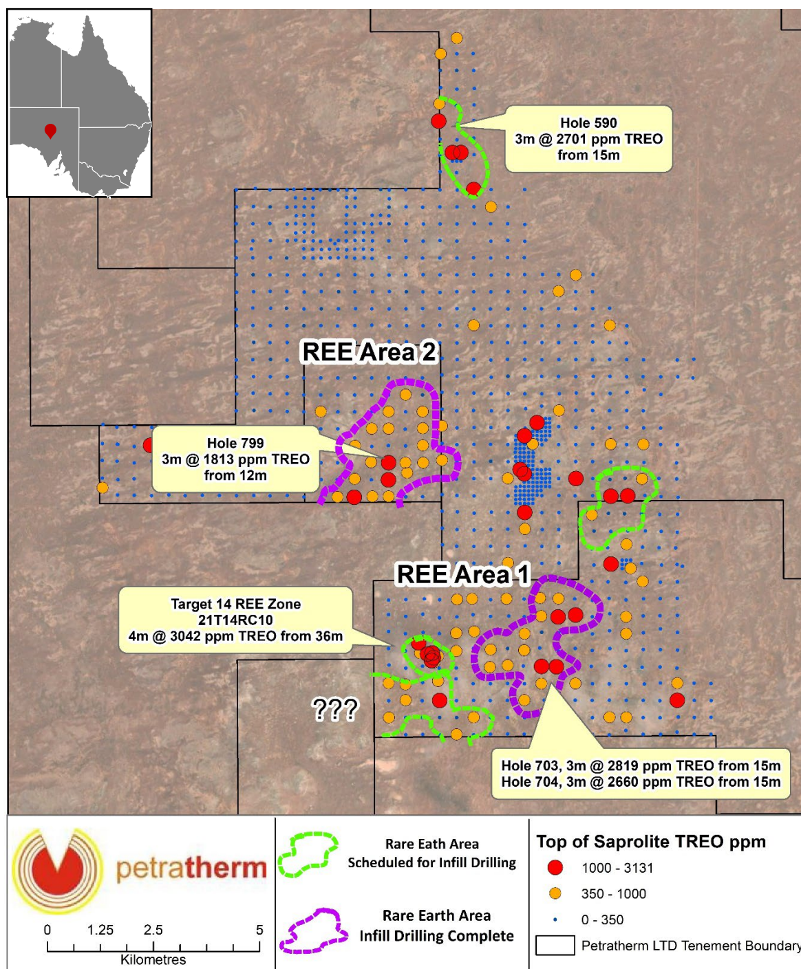
Figure 1 Comet Project REE Results Overview Map
