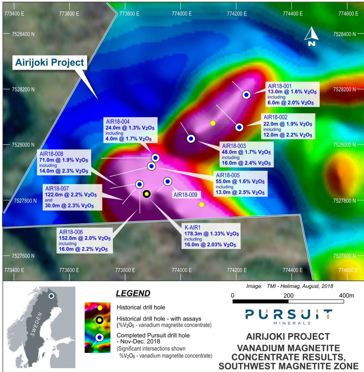
Figure Two – Airijoki Project Southwest Magnetic Zone Summary Drill Hole Results
