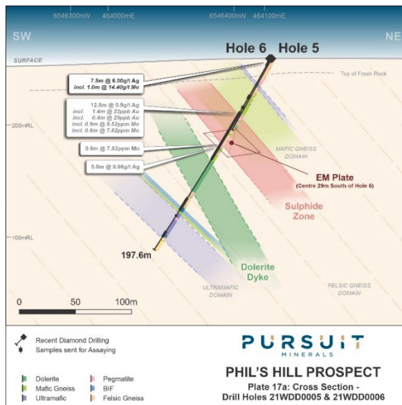
Figure 2: Drill section holes 5 and 6 Phil's Hill
