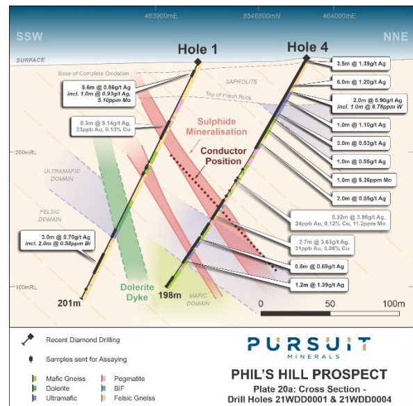
Figure 3: Northern diamond section holes 1 and 4
