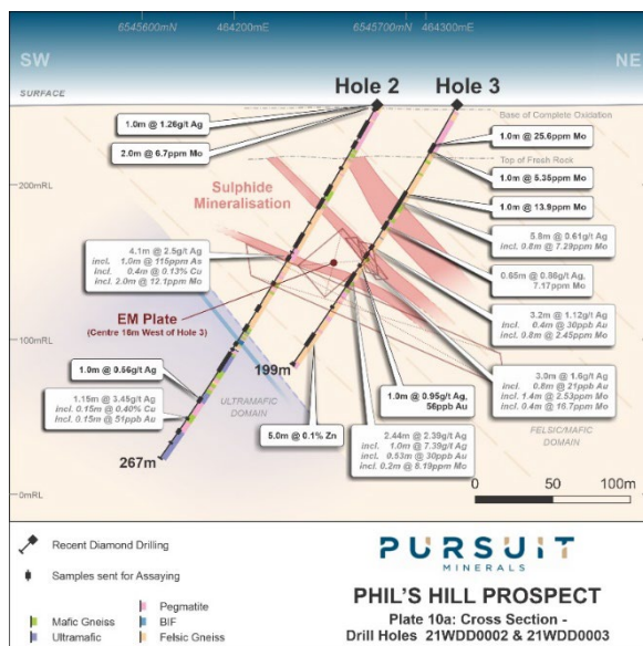
Figure 4: Drill section holes 2 and 3 Phil's Hill
