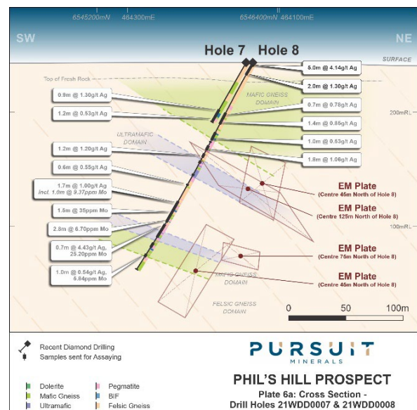
Figure 5: Southern drill section holes 7 and 8 Phil's Hill
