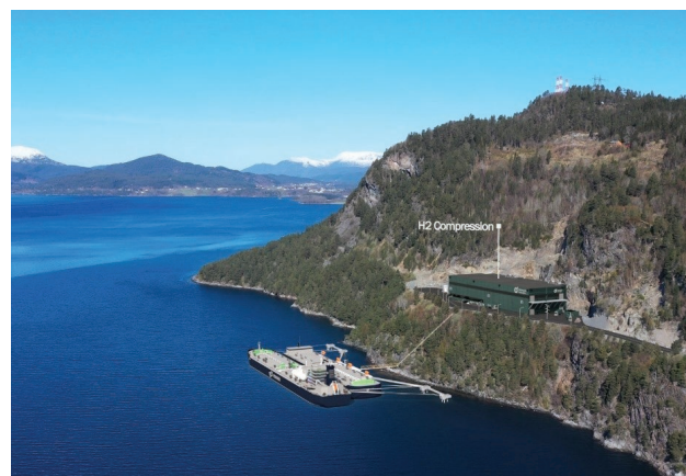
Figure 2 Compression plant located at adjacent site to a dedicated jetty for bulk export using Provaris H2Leo storage barge and H2Neo carrier
