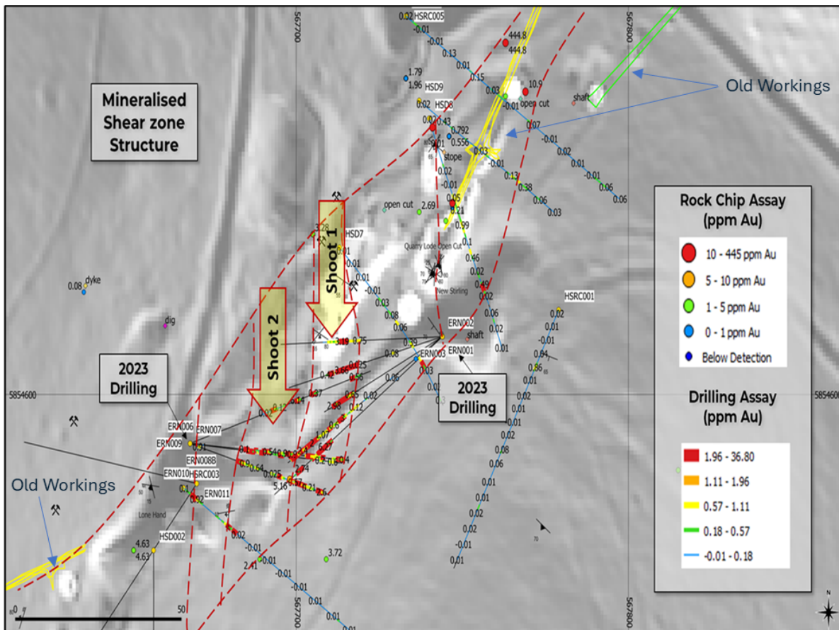
Figure 4: Structural Interpretation against drilling on LiDAR and Multiple Shoot Intersections (inferred by yellow arrows). MGA94 Zone 55.
