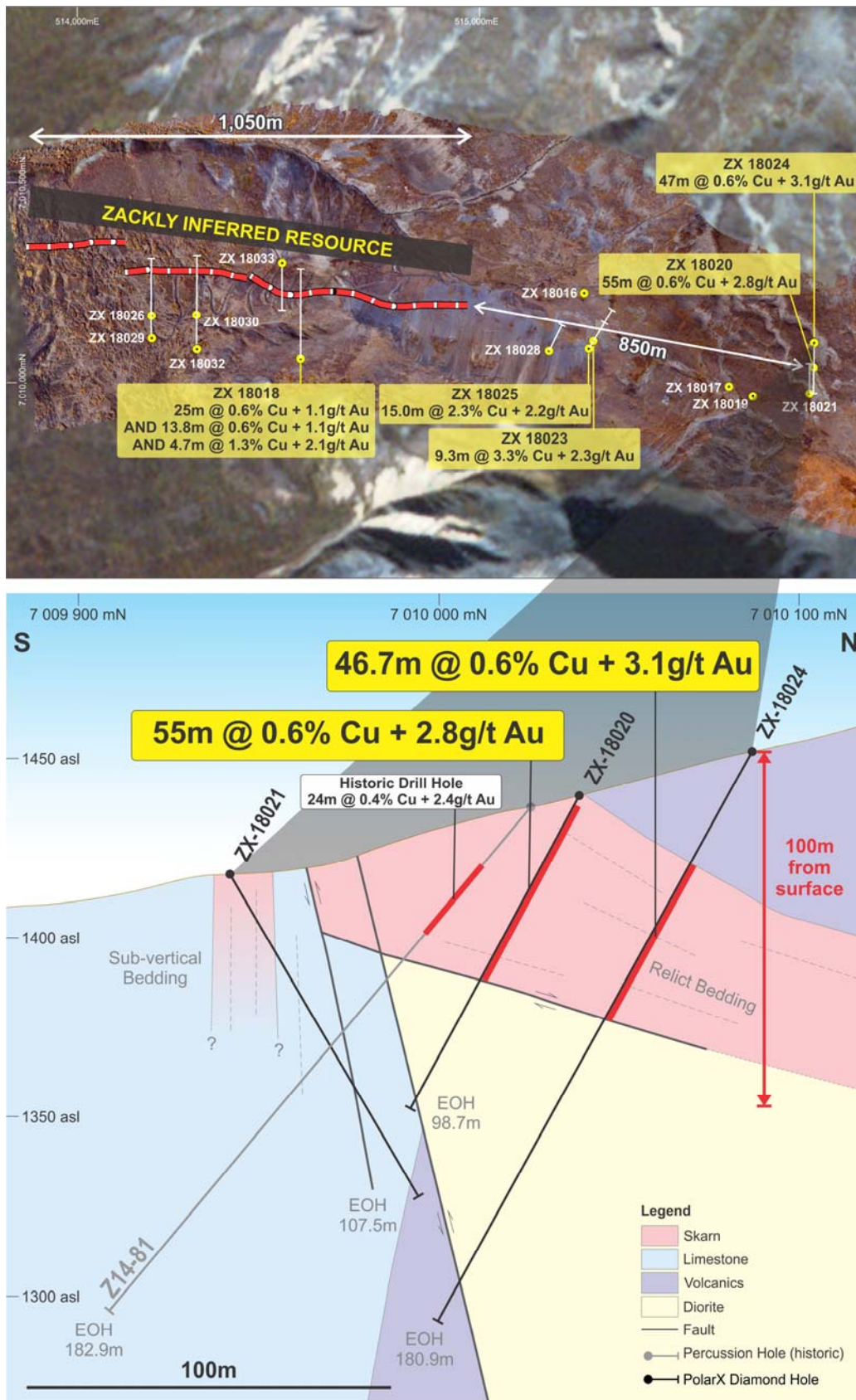
Figure 1. Drill hole plan for Zackly showing the 2017 surface trace of PolarX's inferred resource outline (red) and the 2018 drill holes collared to date (yellow) on detailed drone imagery, with the cross section for holes ZX-18020, ZX-18021 and ZX-18024.
