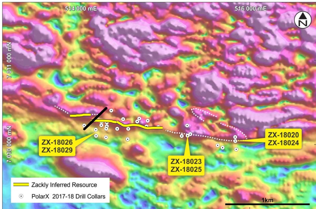
Figure 3 Analytic Signal image processed from the 50m spaced aeromagnetic survey demonstrates a strong association between the mineralisation and the magnetic data at the Zackly Main Skarn resource. It further suggests a continuation to the east skarn mineralisation intersected in holes ZX-18023, ZX-18025 and ZX-18020, ZX-18021 & ZX-18024.
