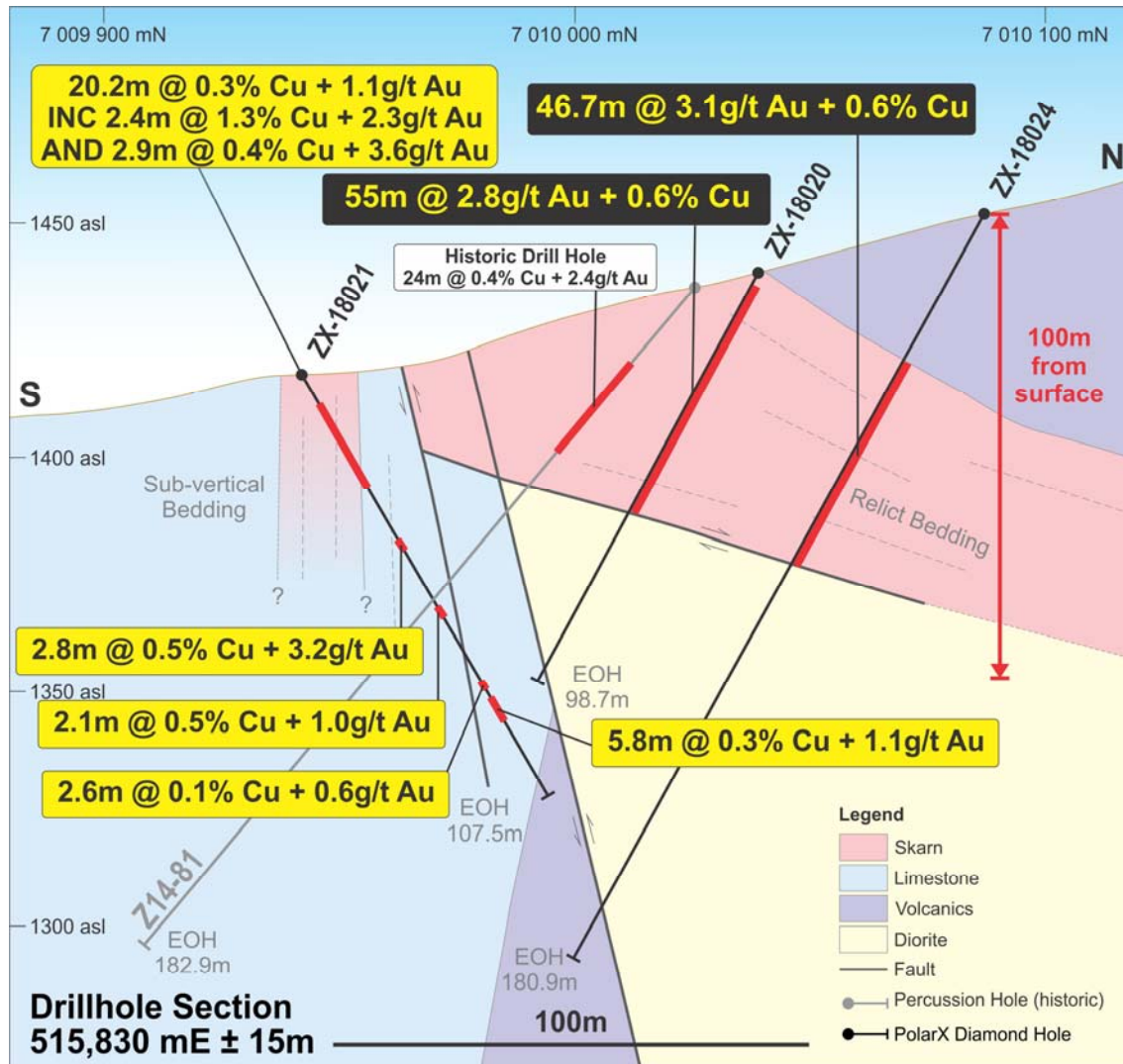
Figure 5 Cross-section showing assay results 850m to the east of the known resource and highlighting thick, near-surface, low angle mineralisation with potential for open pit extraction
