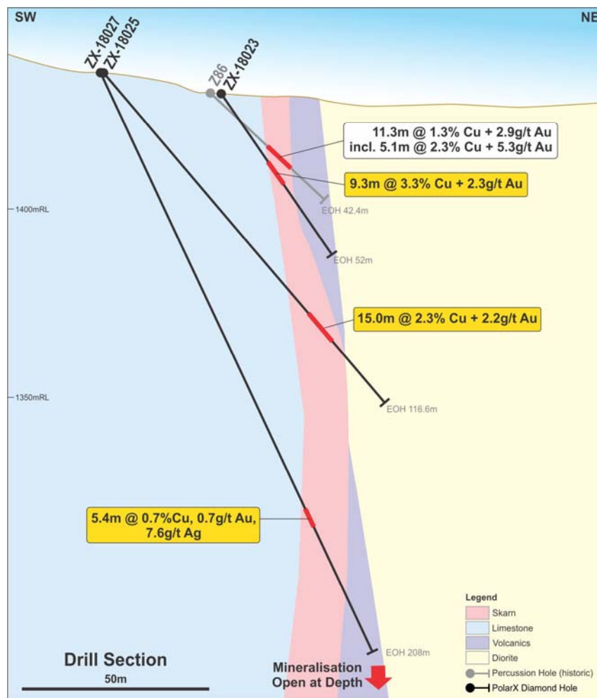
Figure 4 Cross-section showing assay results 350m to the east of the known resource
