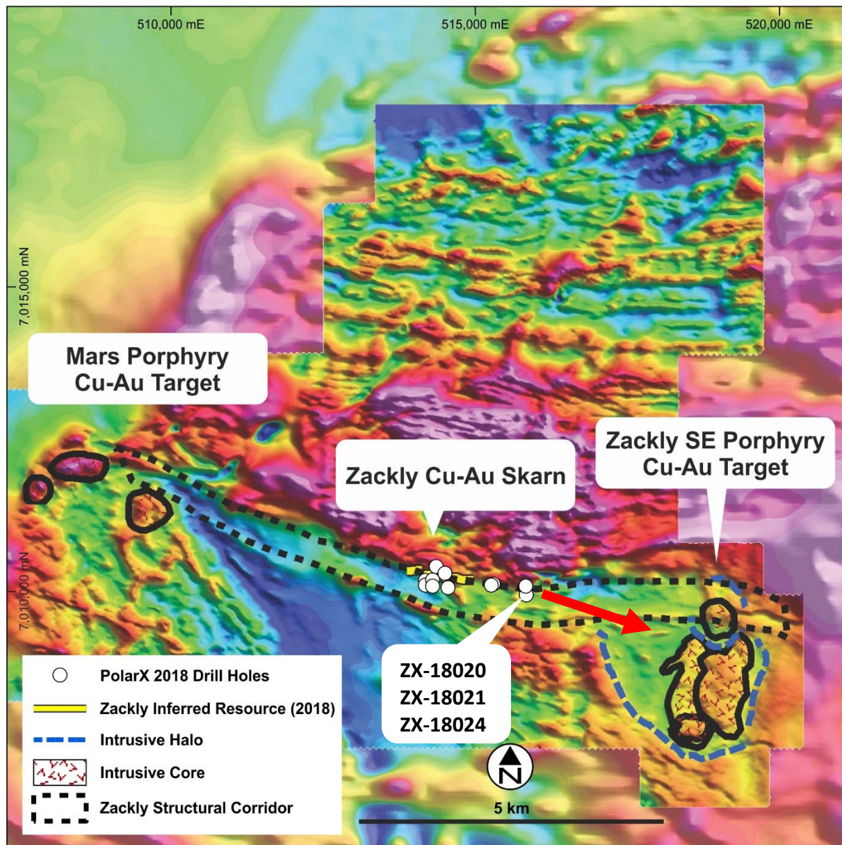
Figure 6 Zackly eastern skarn zone discovered in holes ZX-18020, ZX-18021 & ZX-18024 is situated within an east trending mineralised copper & gold corridor that is 'vectoring' towards a possible mineralised porphyry intrusive complex identified in the 50m line spaced aeromagnetic survey just 2km to the southeast.
