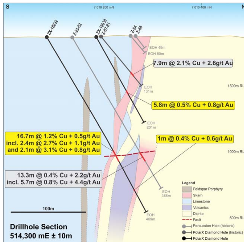
Figure 1 Hole ZX-18032 has intersected multiple copper & gold mineralised zones in skarn commencing near historical drill intercepts. This confirms that mineralisation remains open at depth.
