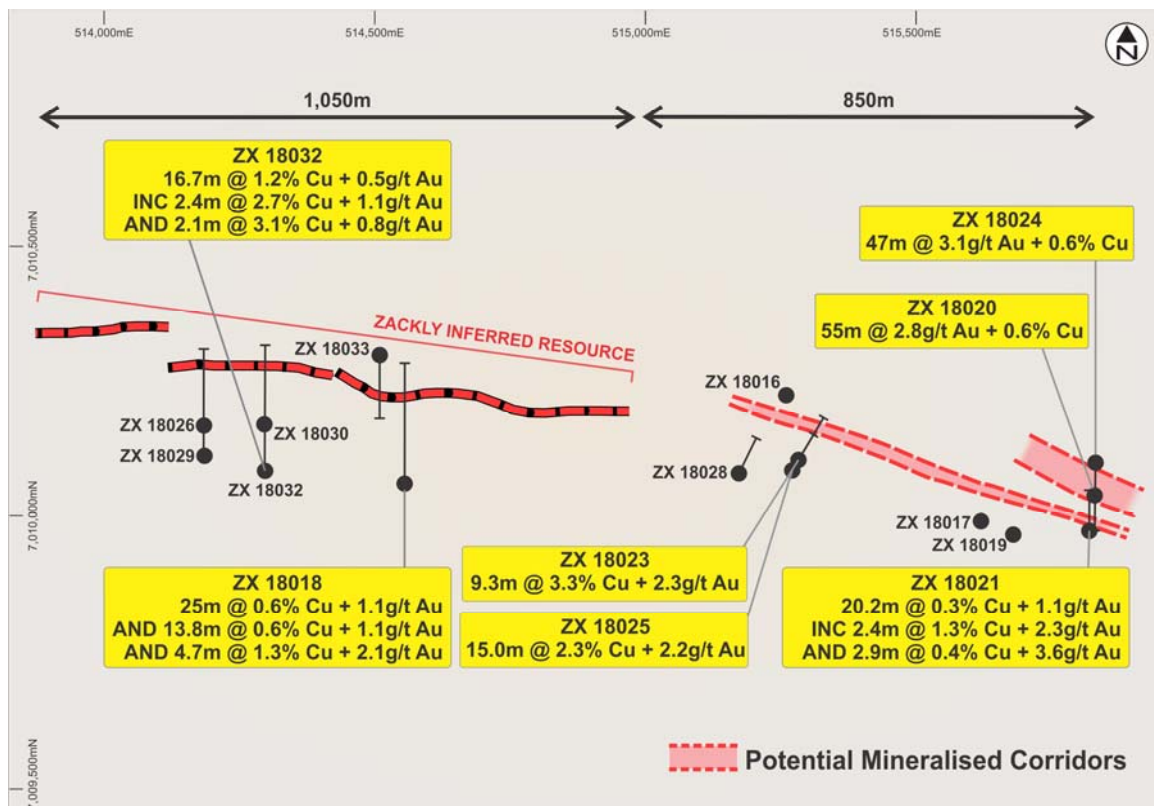
Figure 2 Drill hole plan for Zackly showing the 2017 surface trace of PolarX's inferred resource outline (red) and the 2018 drill hole collars (black), with the cross section for holes ZX-18032, ZX-18020, ZX-18021 and ZX-18024.
