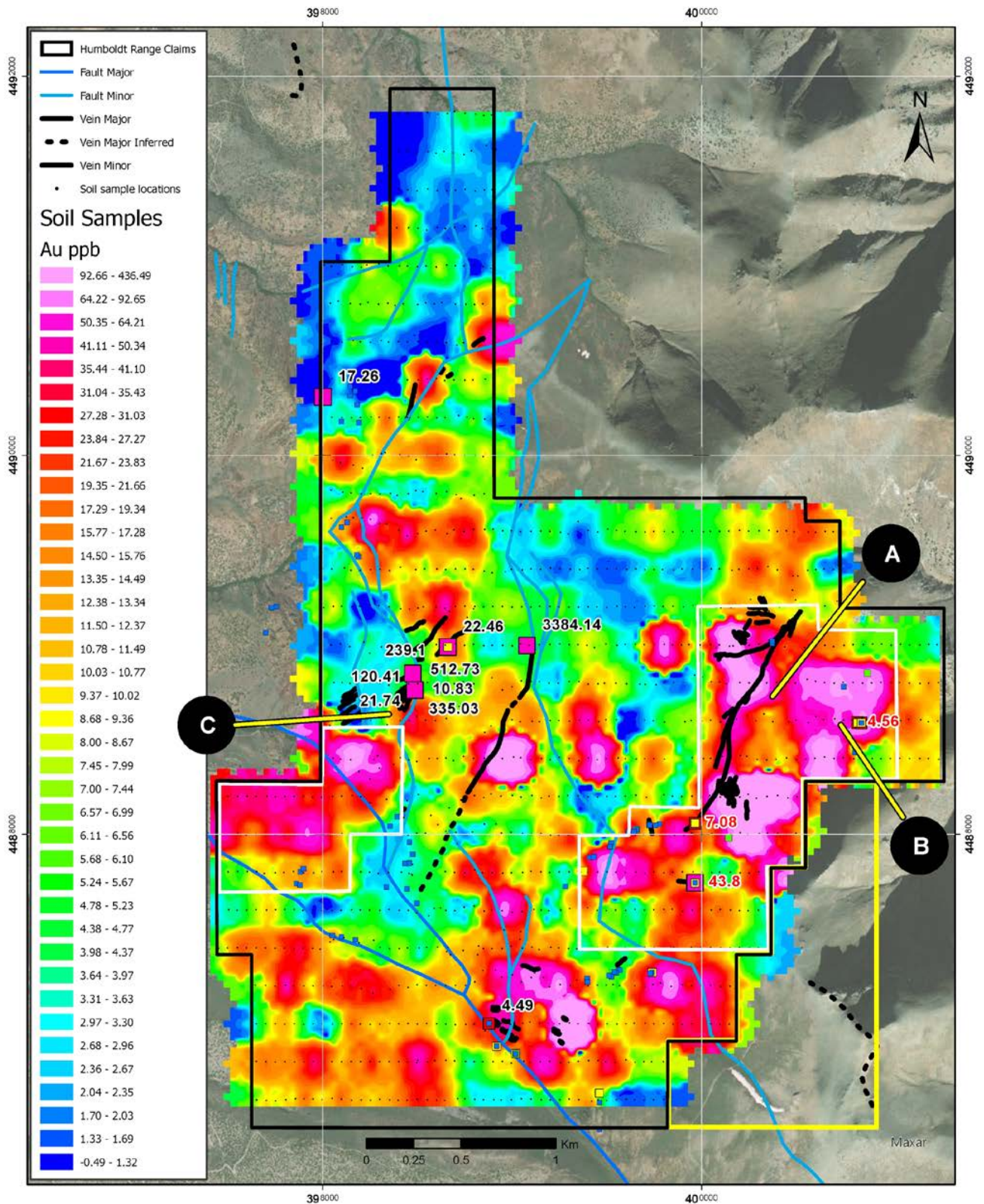
Figure 2. Gridded image of gold in soil sampling overlain with rock-chip sample assays, labelled where >4g/t gold. Yellow box outlines new federal lode claims staked in the SE corner of the project. White boxes denote areas for infill sampling commencing this month, and labels A, B and C denote locations of Figures 3, 4 and 5 respectively in this report.
