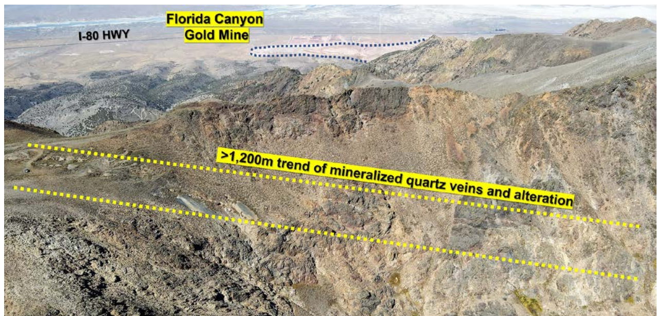
Figure 3 Steep face and ridgeline at the head of Star Canyon showing the extensive scale of large quartz vein array extending across the face. Drill rig access from behind the ridge is possible. The 5M oz Florida Canyon Gold Mine is less than 3km behind at the bottom of the hill.
