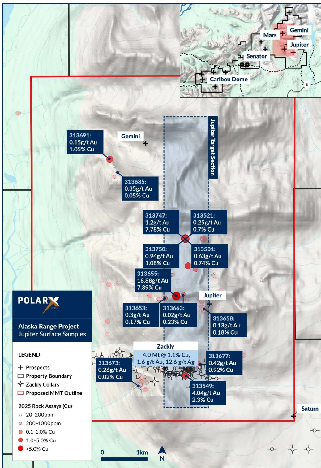
Figure 7. Regional sample results for Copper and Gold on location at the Jupiter, Gemini, and Zackly Deposit areas.
