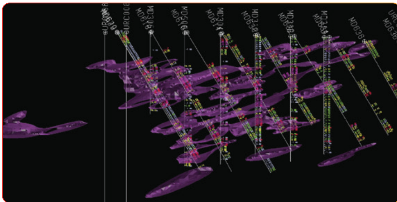
Figure 1: Oblique view looking NW of Uley 2 wireframes and drillholes and connections to Uley 3
