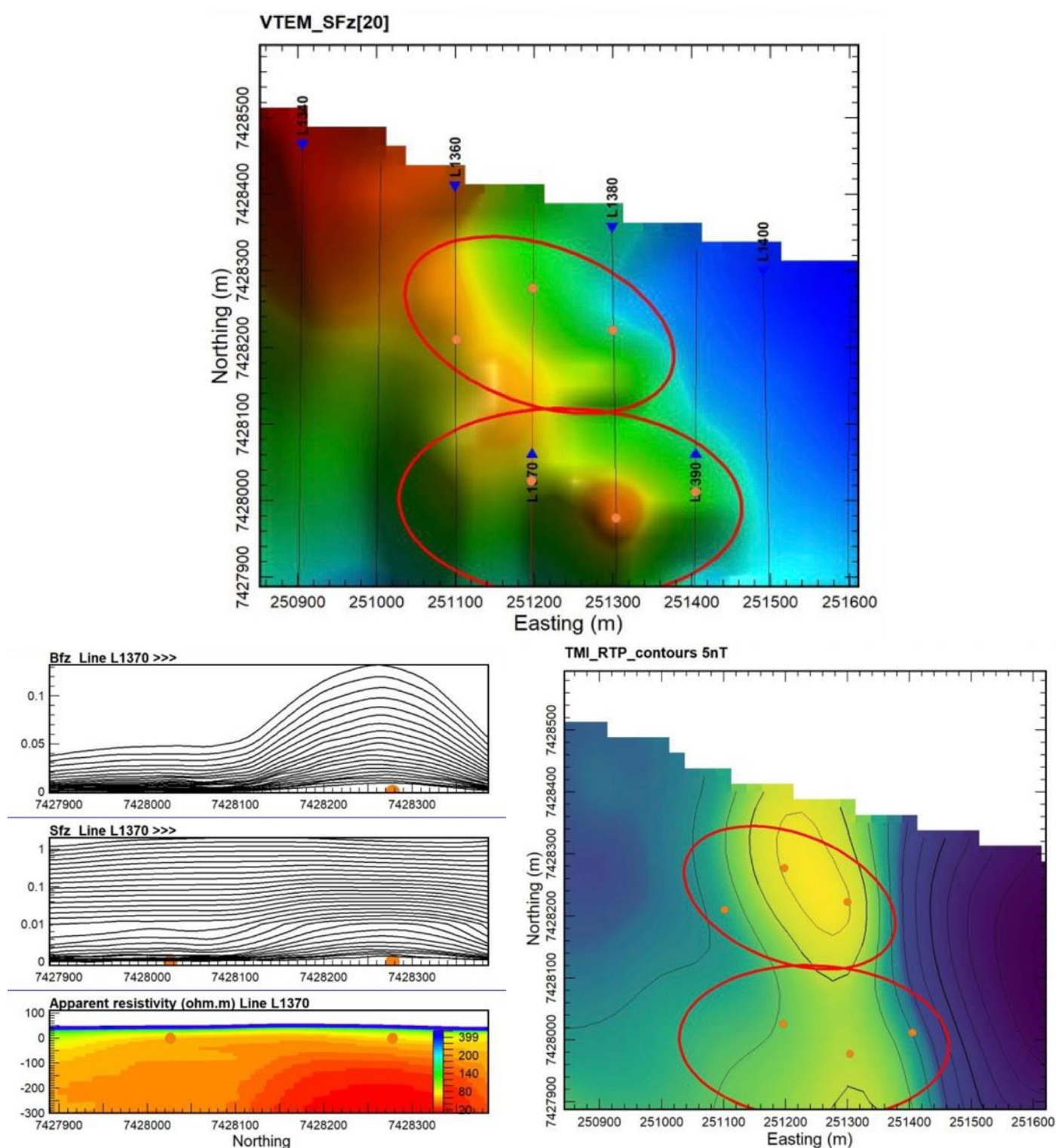
Figure 4: VT-01 VTEM SFz channel 20, Bfz Line 1370, apparent resistivity and TMI RTP contours. VT01 GDA94 MGA65.
