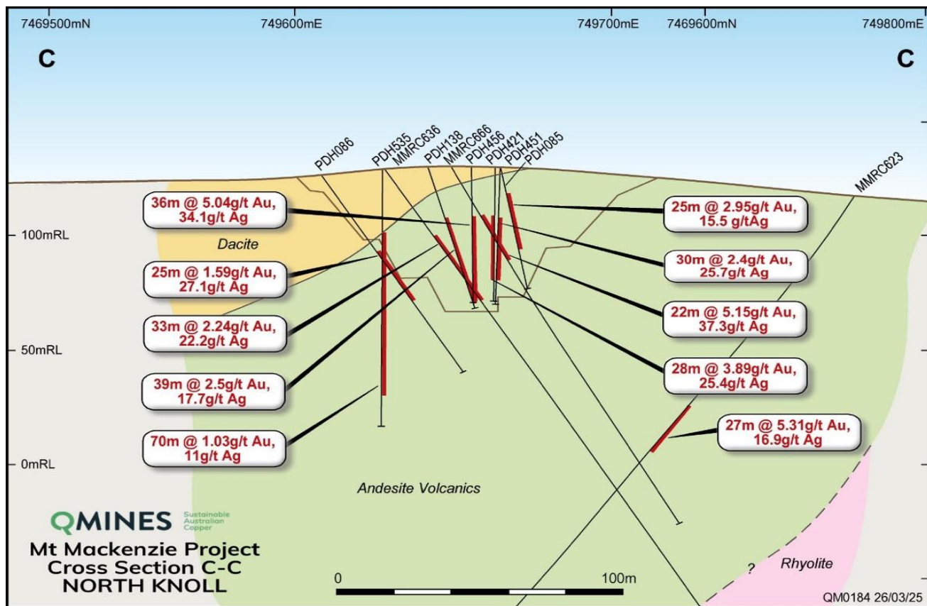
Figure 5: Section CC from North Knoll at the Mount Mackenzie project. (NB – pit shell shown here is from historic optimisation)
