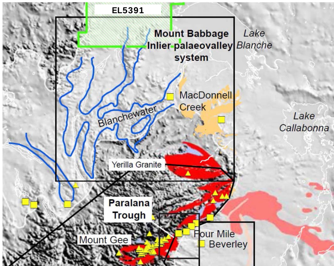
Figure 20: Plan showing interpreted Blanchewater Palaeovalley and EL 5391 (Geoscience Australia).
