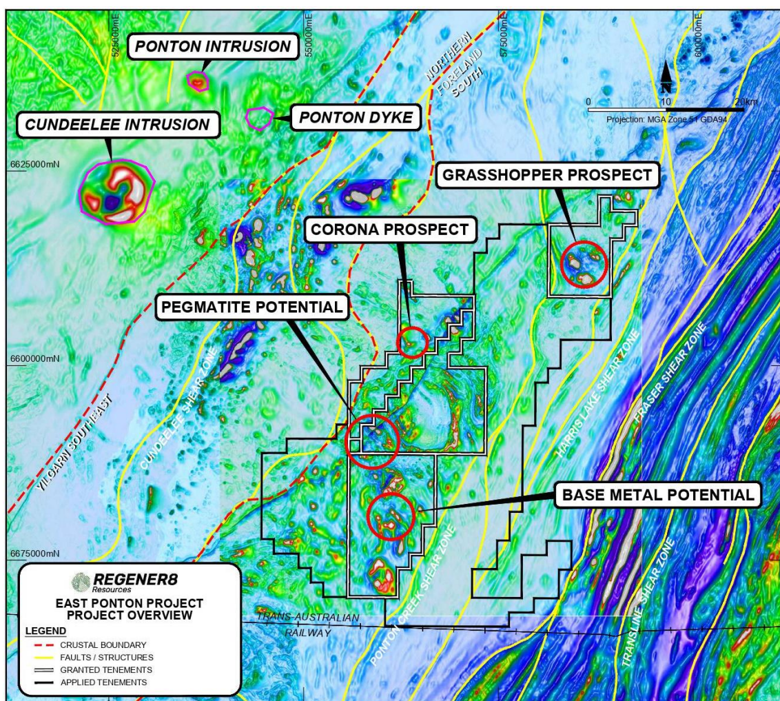
Figure 2: East Ponton Project, Optioned and Applied tenements with prospect potential, over Regional Geological and Total Magnetic Intensity
