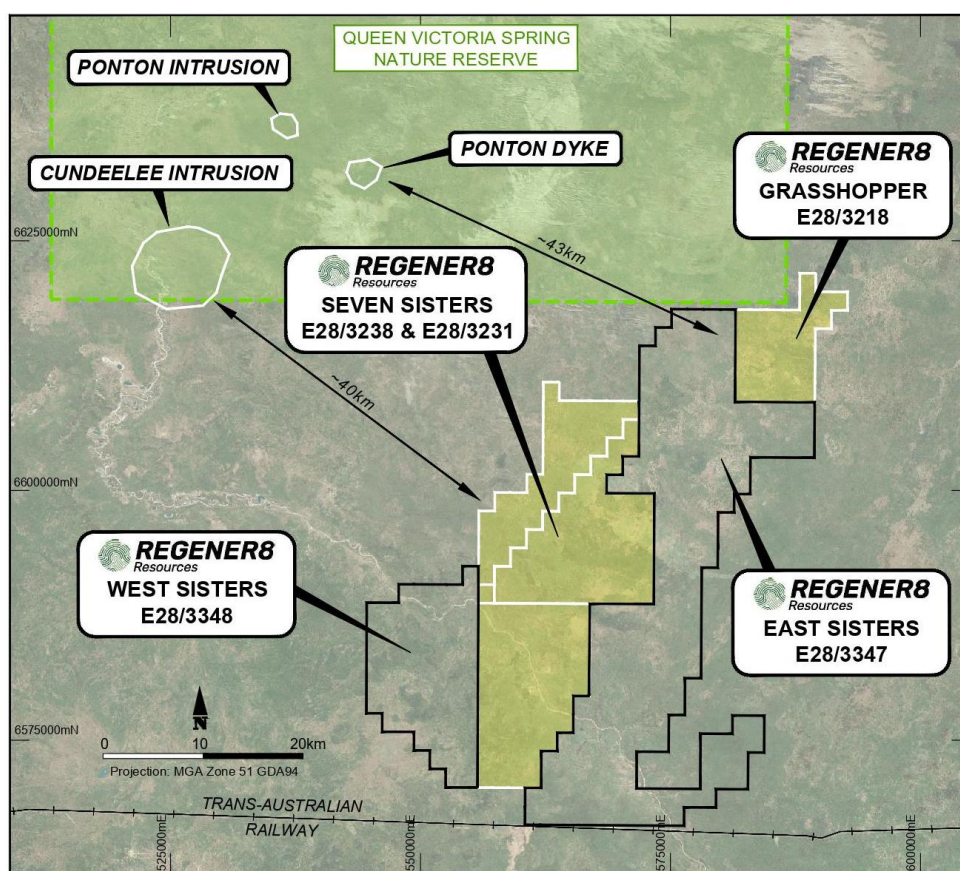
Figure 1: East Ponton Project with Optioned and Applied Tenements
