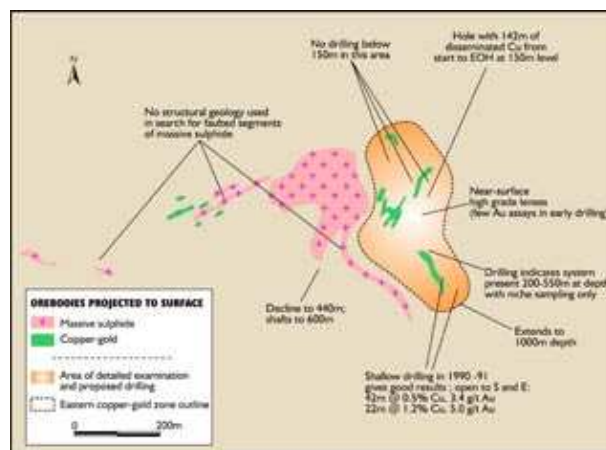
Falun Copper-Zinc Mine - orebody projected to surface
