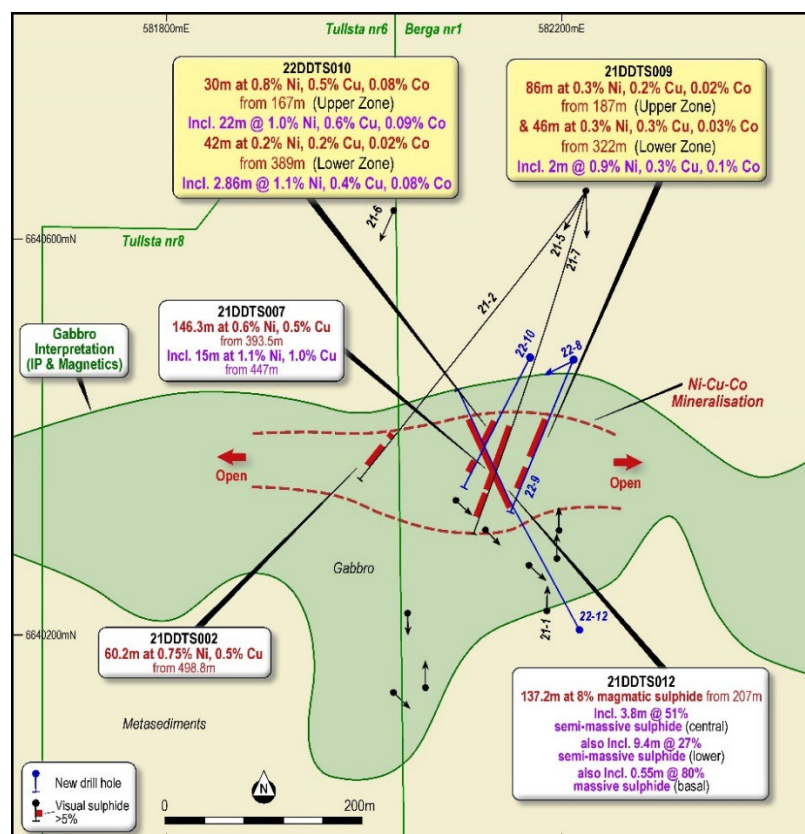
Figure 2: Simplified interpreted bedrock geology map of the host gabbro intrusion at Granmuren and highlighted drilling intersections.
