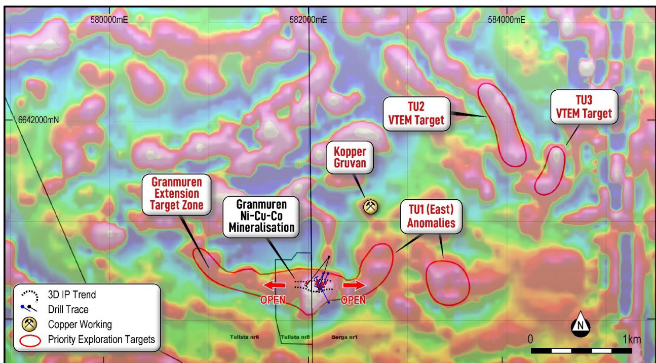
Figure 4: Plan view of the Ragnar tenure of 1 st Vertical Derivative VTEM magnetic image showing surface projection of Ni-Cu-Co mineralisation interested to date at Granmuren as well as other regional and/or VTEM targets.
