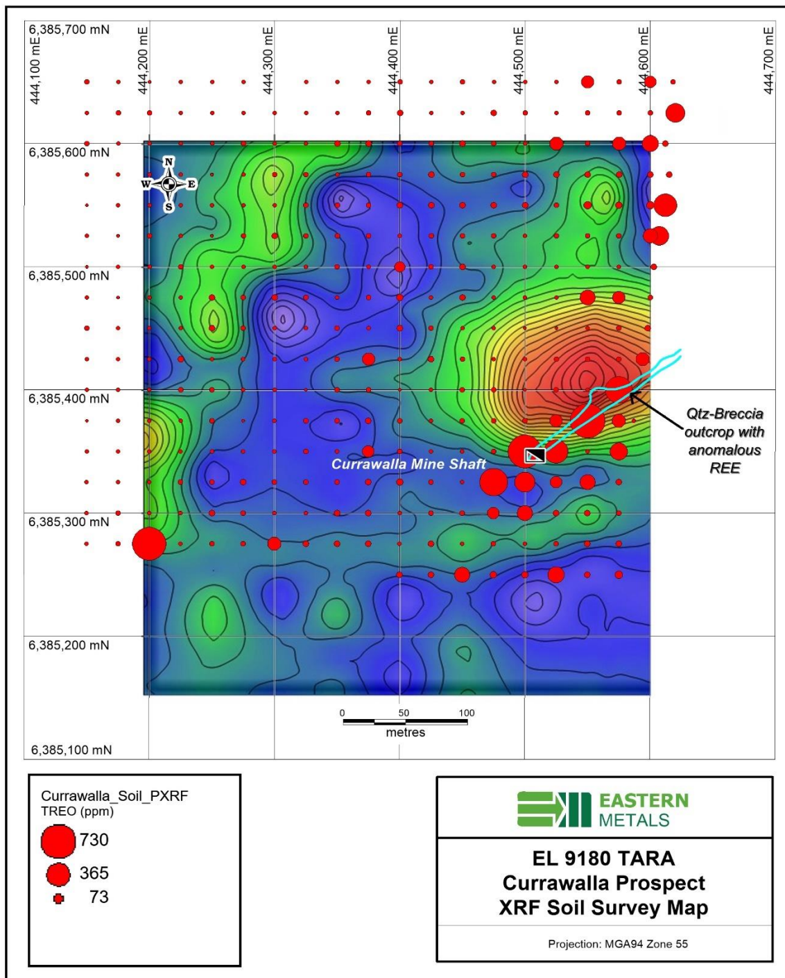
Figure 2. Soil Sampling Geochemistry, Currawalla Prospect
