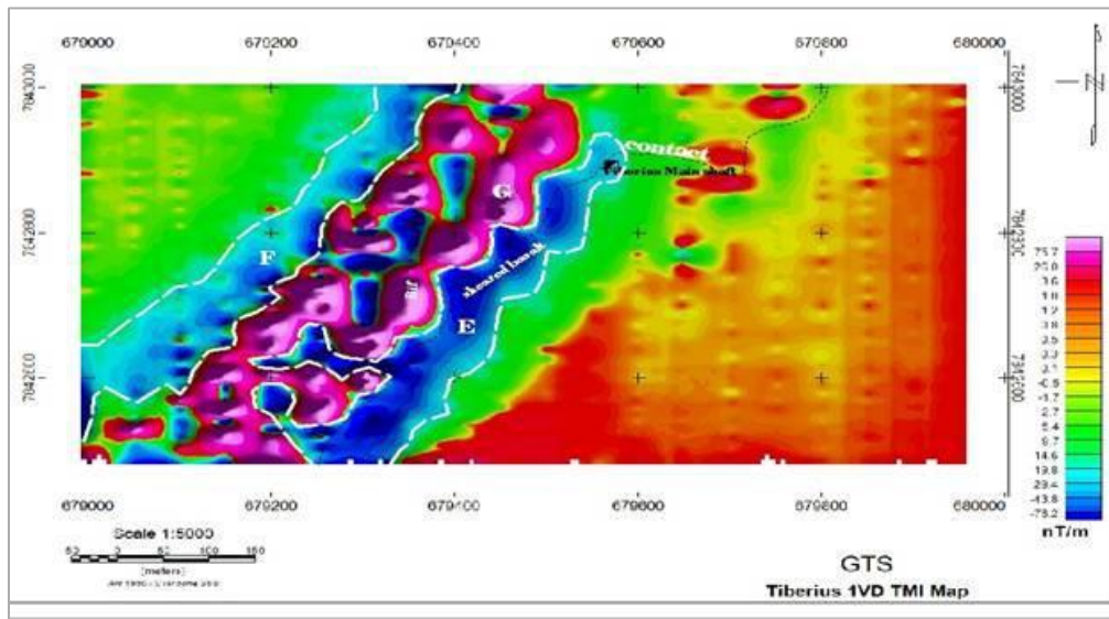
Figure 2. Lonely Mine Gold Project – Tiberius Prospect 1st Vertical Derivative Map
