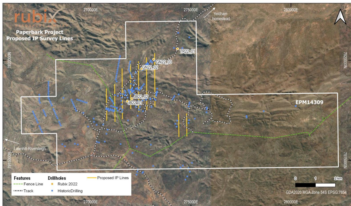
Figure 4 – Planned IP survey lines at the Paperbark Project
