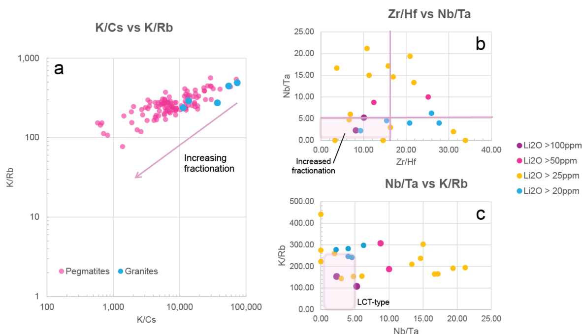
Figure 3 –Geochemical discrimination diagrams for the Ceiling Project, showing with fractionation trends and fertile fields.
