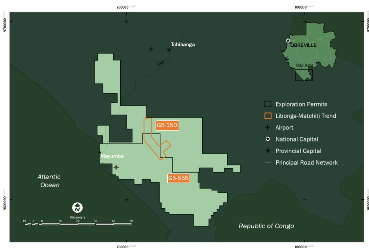
Figure 1: Tenement map for the Nyanga Project. Datum UTM WGS84 32S. Source: AMM.
