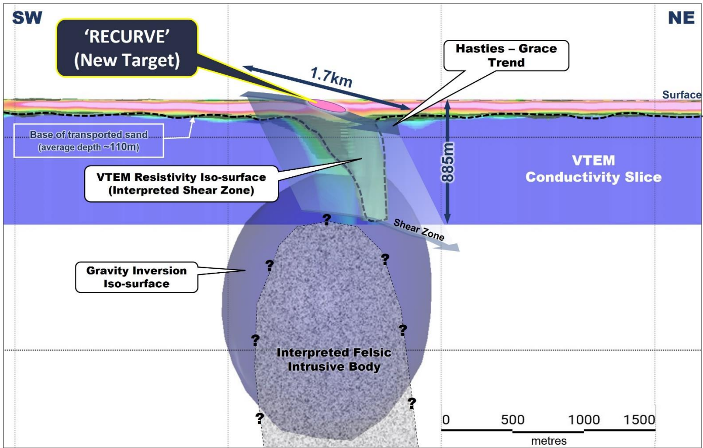
Figure 3: Schematic section through Recurve Target.
