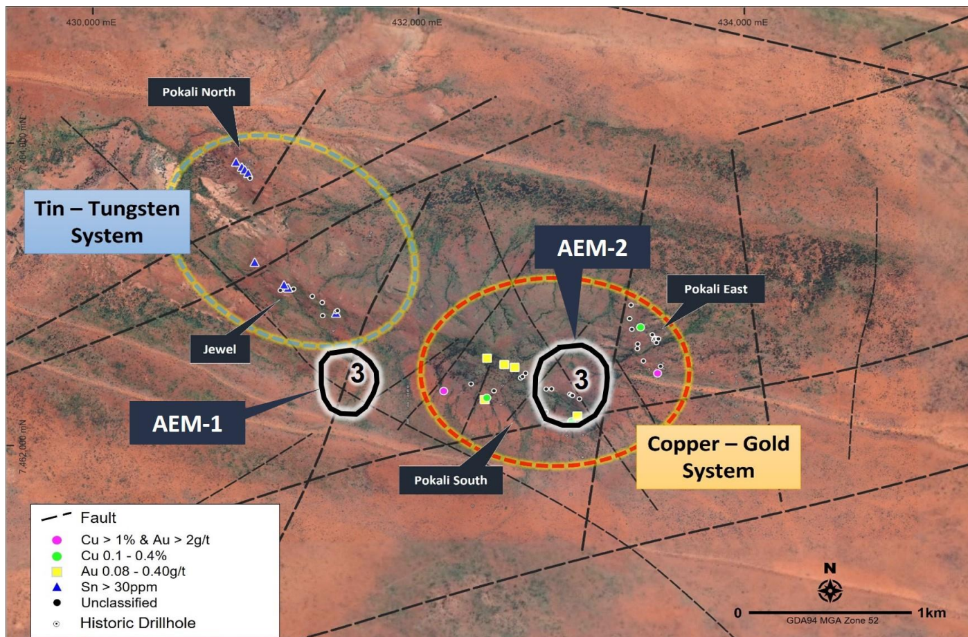
Figure 4: Classified rock-chip samples highlighting two discrete mineral systems and location of AEM-1 and AEM-2 anomalies.
