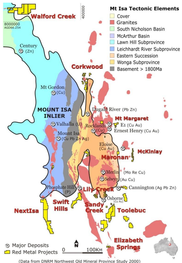
[Figure 6] Mount Isa Inlier: Red Metal projects and regional geology showing extent of the outcropping Proterozoic rocks, main granite intrusions and major deposits of the region.
