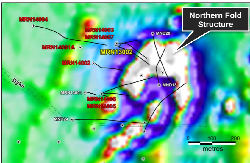
[Figure 2] Maranon Project: Drill hole location plan showing current holes around the lead-sulphide mineralisation in MRN13002 (yellow). Drill holes MRN14001A, MRN14002, MRN14003, MRN14005, MRN14006 and MRN14007 are evaluating the shallower ore potential around MRN13002. MRN14004 is testing the potential of the system to zone towards semi-massive sulphides at depth. Drilling is in progress.
