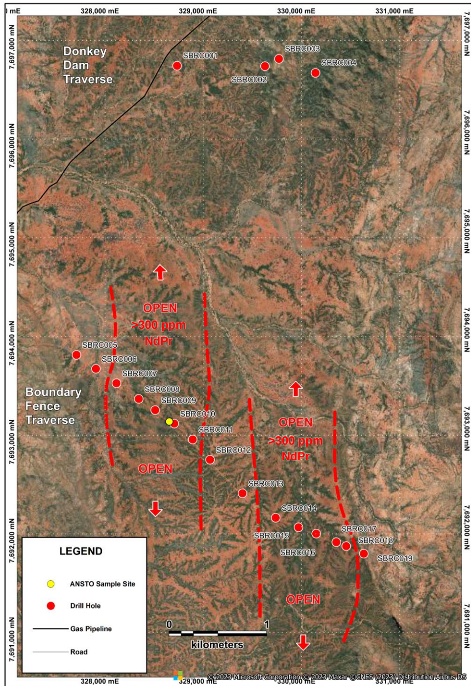
[Figure 1] Sybella Project: Recent Red Metal drill hole locations on satellite image highlighting wide zones of >300 ppm NdPr oxide. ANSTO surface sample site used for mineralogical and preliminary leach test highlighted as yellow circle.
