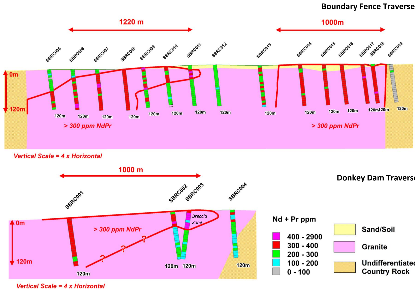
[Figure 2] Sybella Project: Drill sections showing variation in NdPr oxide values at depth and between holes for two traverses across the granite.
