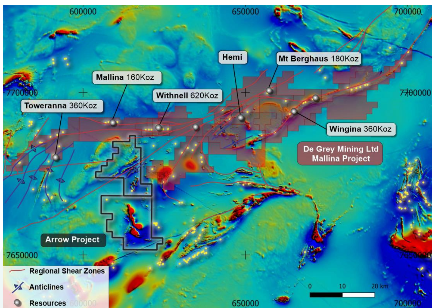
Figure 1: Arrow Project – ASX: DEG Tenure, Regional Shear Zones and Resources
