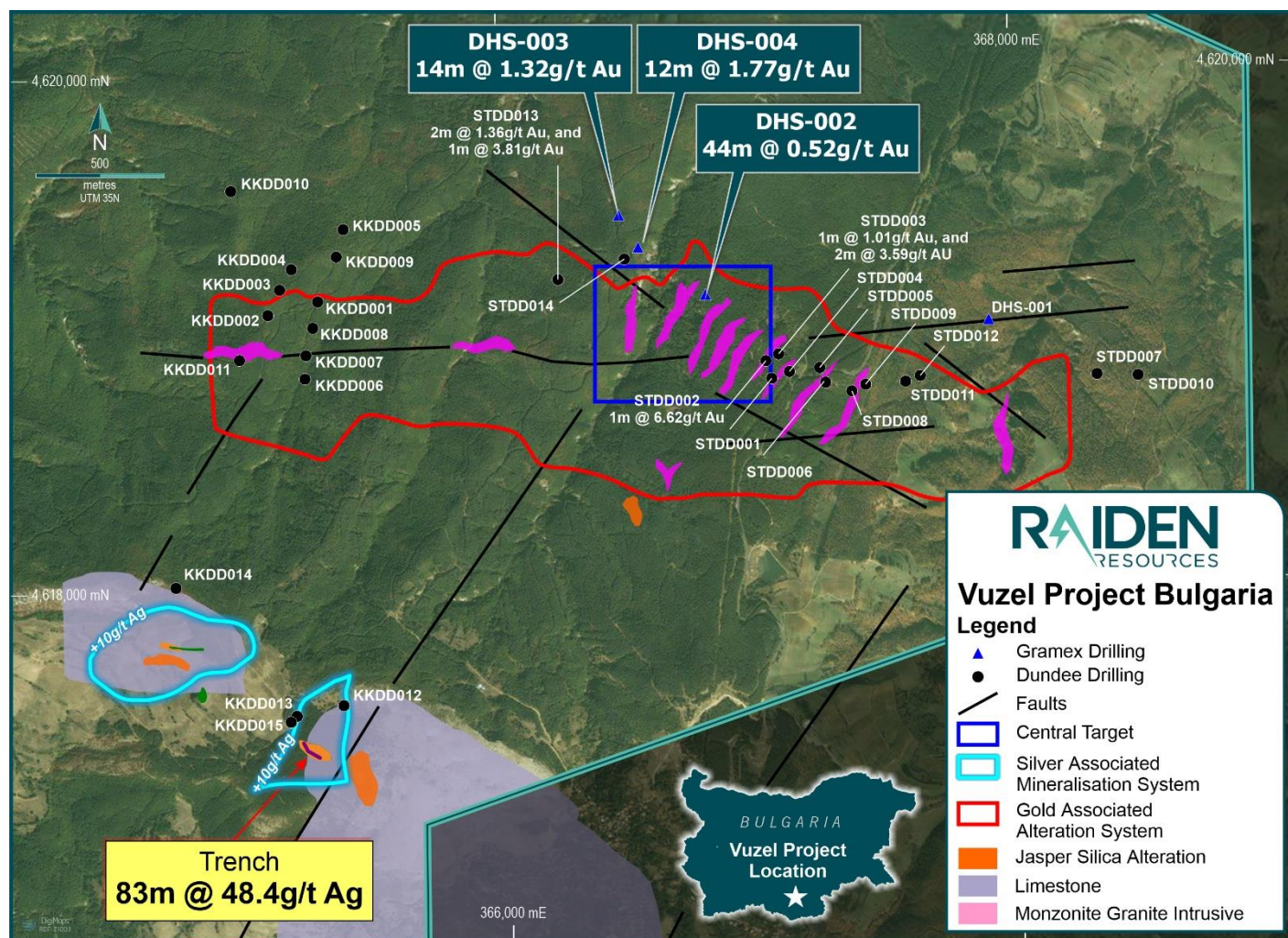
Figure 1 – Location of the historical silver soil anomalies and the trench with the high Ag values, in relation to the main gold anomaly zone.
