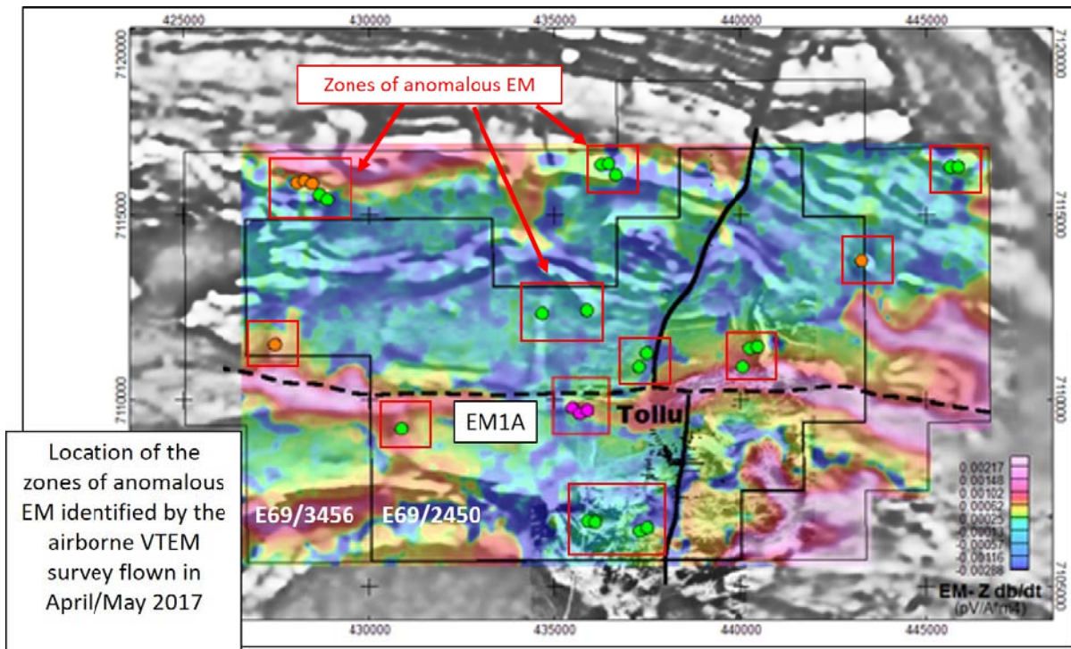
Figure 2 – Location of EM anomalies in relation to the Tollu structural corridor. Tenement E69/2450 airborne magnetic image (grey) with late time Z component channel 48 (10.667 msec after turn off) as the colour image.
