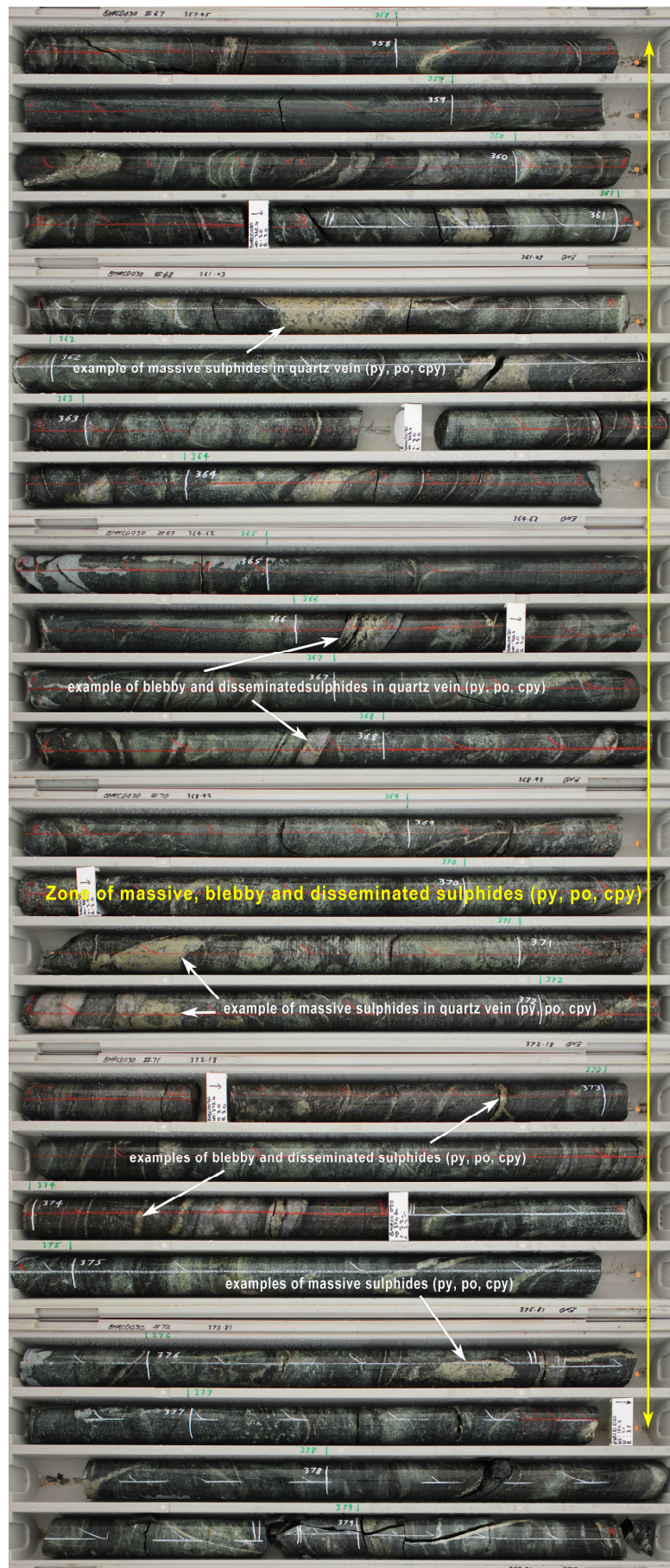
Figure 3: Drill core from 357.45 – 379.41m BHRCD030, showing massive, blebby and disseminated sulphides
