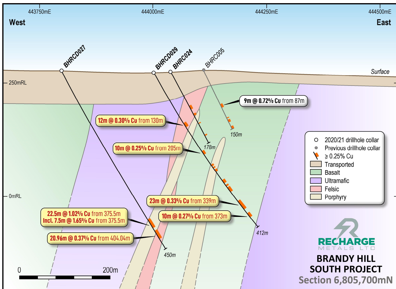
Figure 2. Cross section (refer to Figure 1) showing the significant intercepts in drillholes BHRCD027 and BHRCD029 and previous drilling at the Brandy Hill South Prospect.
